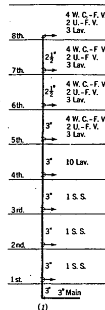
FIG. 5. UP-FEED SYSTEM
