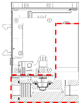
Cross-sectional view of the product
