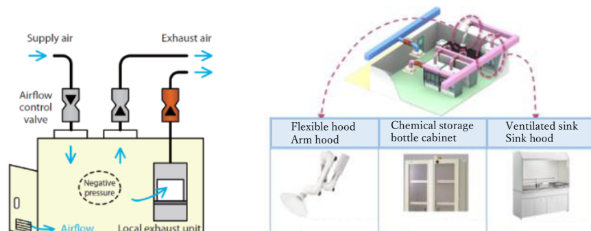
Figure 57 Example of air volume control in a chemical/ Other exhaust applications
