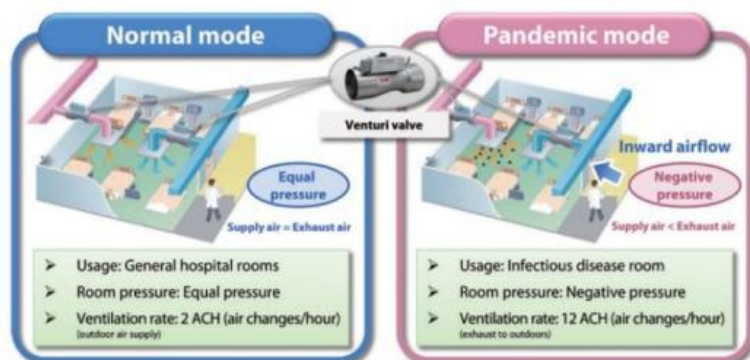
Figure 58 Image of negative and positive pressure control in a hospital room
