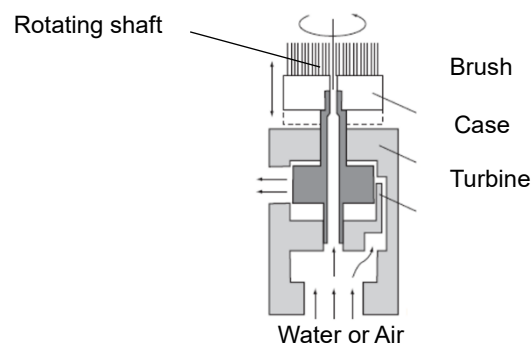
Figure 11 Bearing used for the rotating shaft sliding part of the sensor cleaning brush
