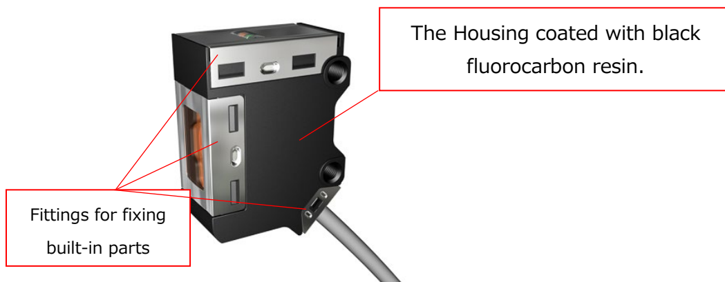
Figure 32 External View/ Detection of workpiece seating in machine tool
