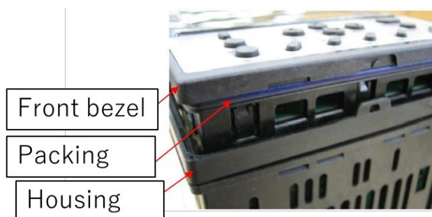
Figure 48 Packing installation explanatory diagram
