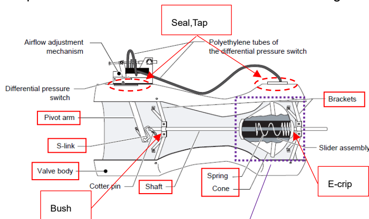
Figure 59 Valve image
