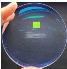
polydimethylsiloxane
