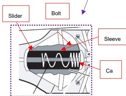
Figure 60 Slider assembly
