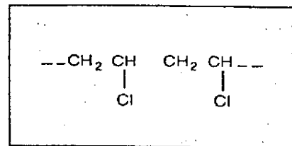
Fig 2.—Polyvinyl chloride.
