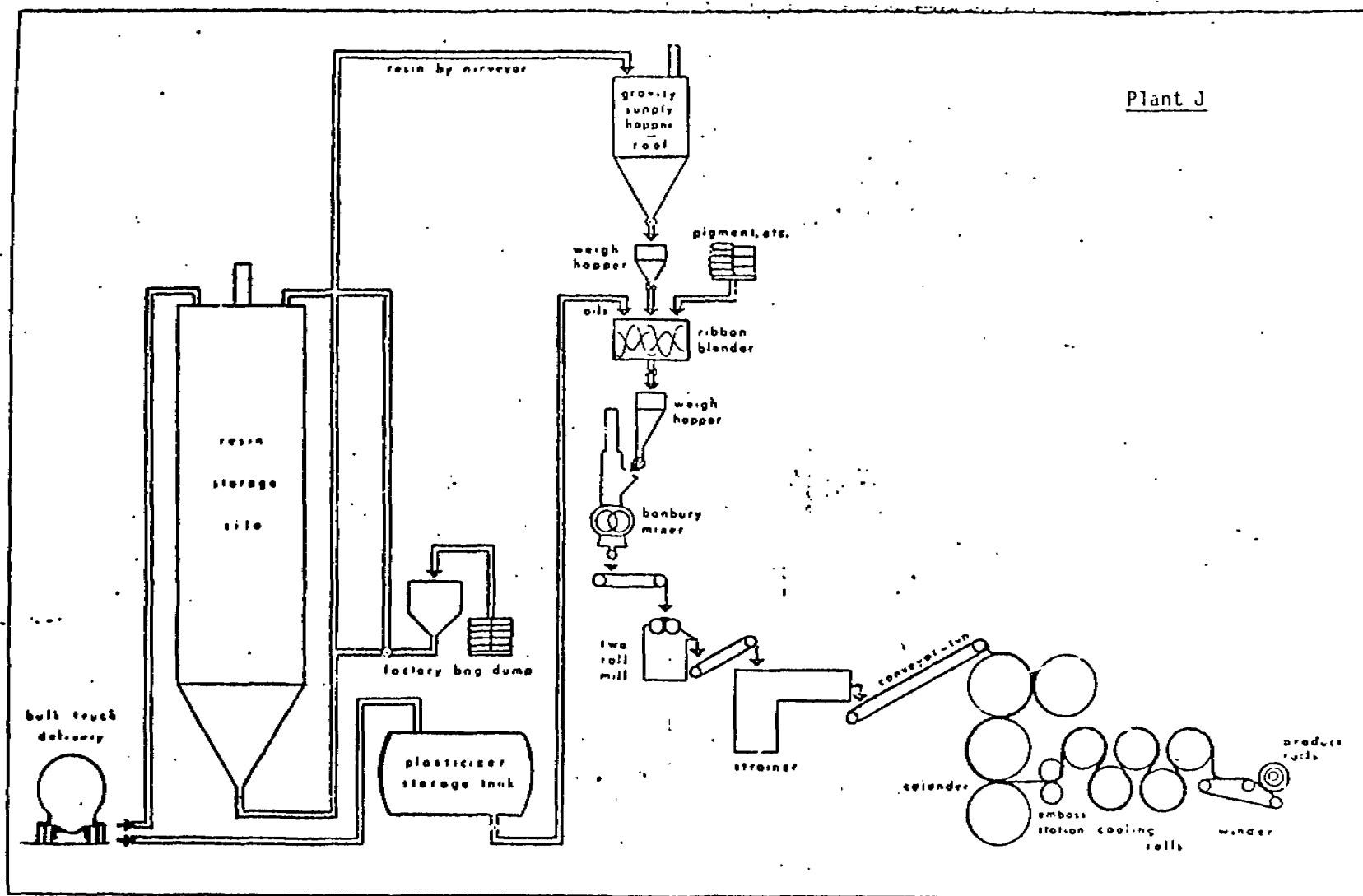
Figure 14. Flow Schematic, Calendered Film Production, Plant J
