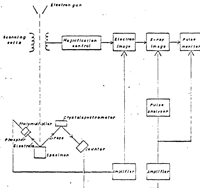
FIG. 1. Schematic diagram of microanalyzer.
