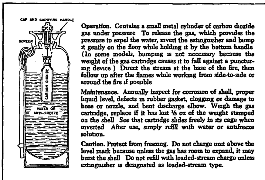
Fig. 34-15. Gas cartridge water extinguisher. May be labeled "loaded stream" if charged with a special alkali-metal salt solution instead of water.
