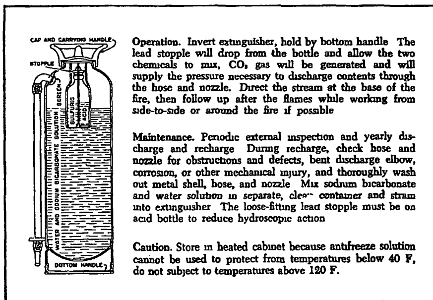
Fig. 34-16. Soda-acid fire extinguisher.
