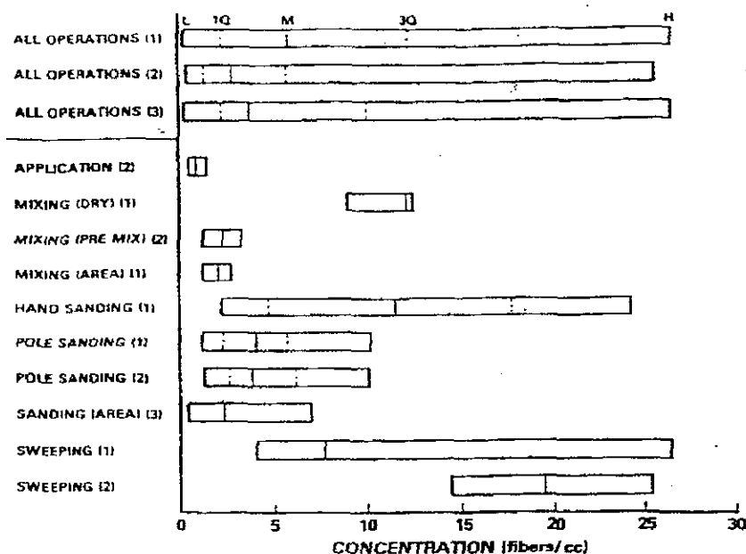
Figure 1 - Observed fiber counts for the various operations in the taping process. The numbers in parentheses (ordinate labelling) refer to the collection time and place as explained in footnote a of Table I. L, 1Q, M, 3Q and H represent Low value, the Lower Quartile, the Median, the Upper Quartile and the High value respectively.
