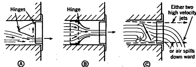
FIG. 14. EFFECT OF VARIOUS DAMPER ARRANGEMENTS DESIGNED FOR STRAIGHT BLOW
