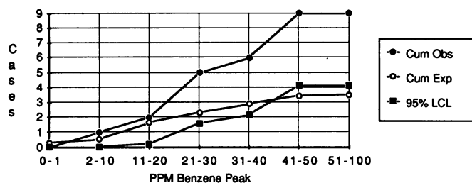
FIGURE 8. Benzene-leukemia dose relationship by peak benzene level (ppm) of Rinsky (5) for all known 1940-1965 Pliofilm workers.
