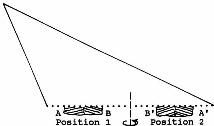
Figure 6. Effect of sample spinning on crystallite diffraction.
