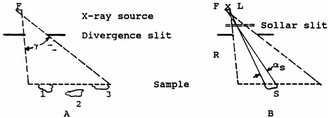
Figure 5. A. Diffractometer optics for incident rays. B. Effective ray paths for a single crystallite.
