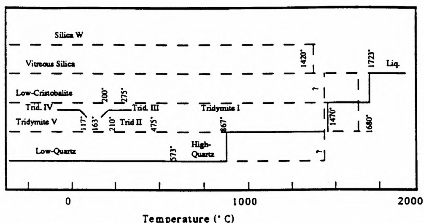
Figure 2. Metastability behavior of \text{SiO}_2 at ambient pressure.
