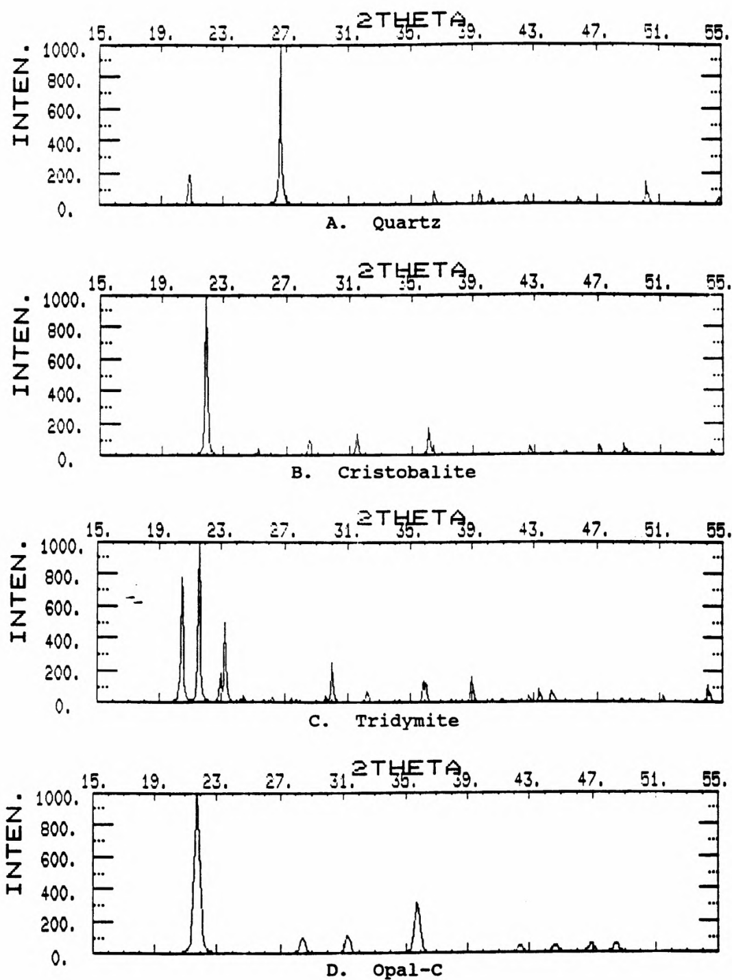
Figure 3. Diffraction patterns of the principal crystalline silica minerals. A. Quartz. B. Cristobalite. C. Tridymite. D. Opal-C.
