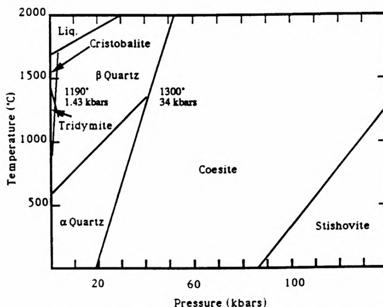
Figure 1. Pressure-temperature phase relations for \text{SiO}_2
