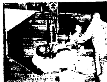
Figure 6. The centrifugal force created by this grinding wheel causes the generated dust to travel in a well-defined path. To prevent dispersion of the dust, the exhaust hood is placed directly in the dust stream, close to its source. (Courtesy American Foundrymen's Society)
