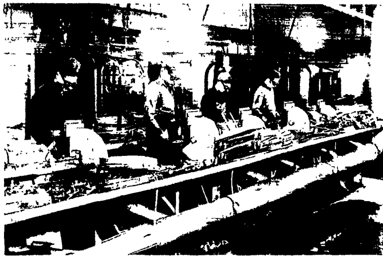
Figure 3. Each of these grinding wheels is partially enclosed by an exhaust hood. Efficient local exhaust is achieved by drawing the dust into the hoods, through branch ducts, and into a central duct which leads to the collection point. (Courtesy American Foundrymen's Society)
