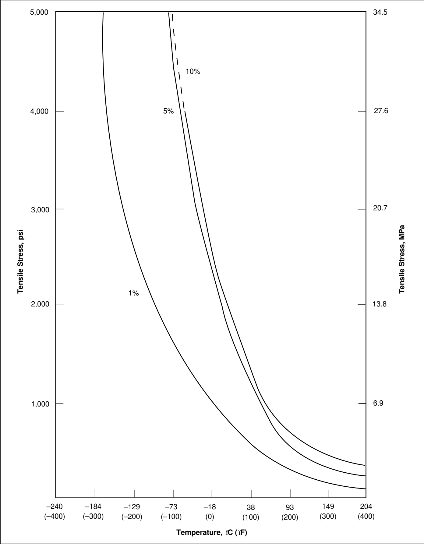
Figure 3. Tensile Stress vs. Temperature at Constant Strain
