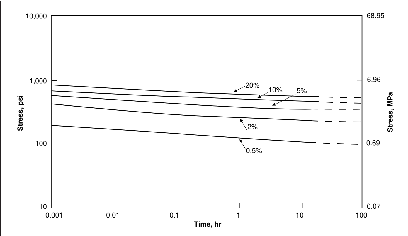
Figure 10b. Tensile Strength Relaxation at 100°C (212°F)
