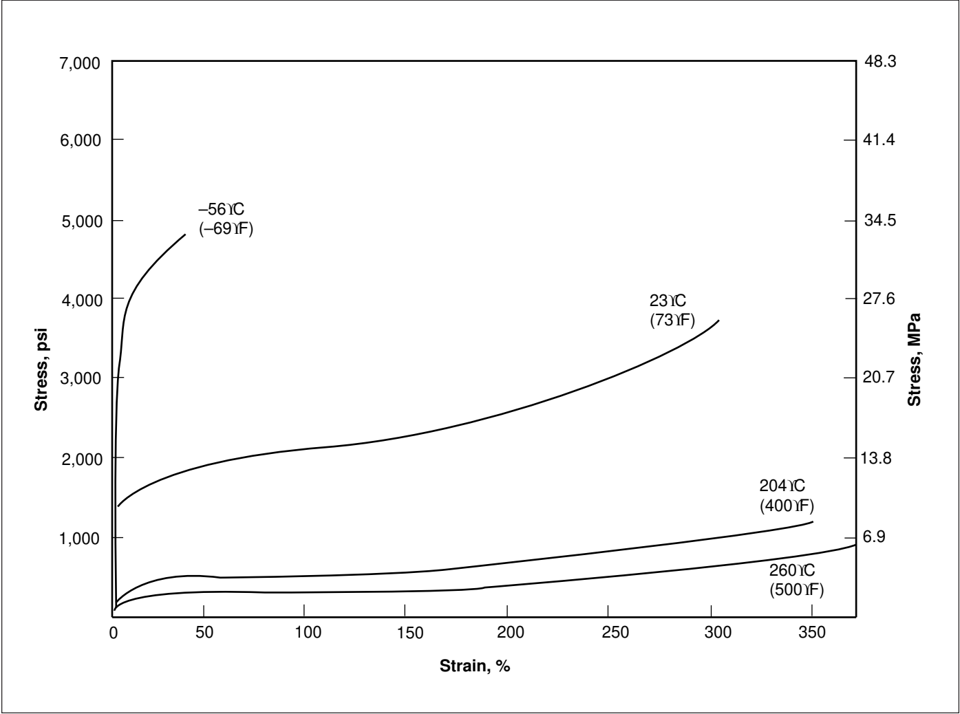
Figure 2b. Stress vs. Strain in Tension
