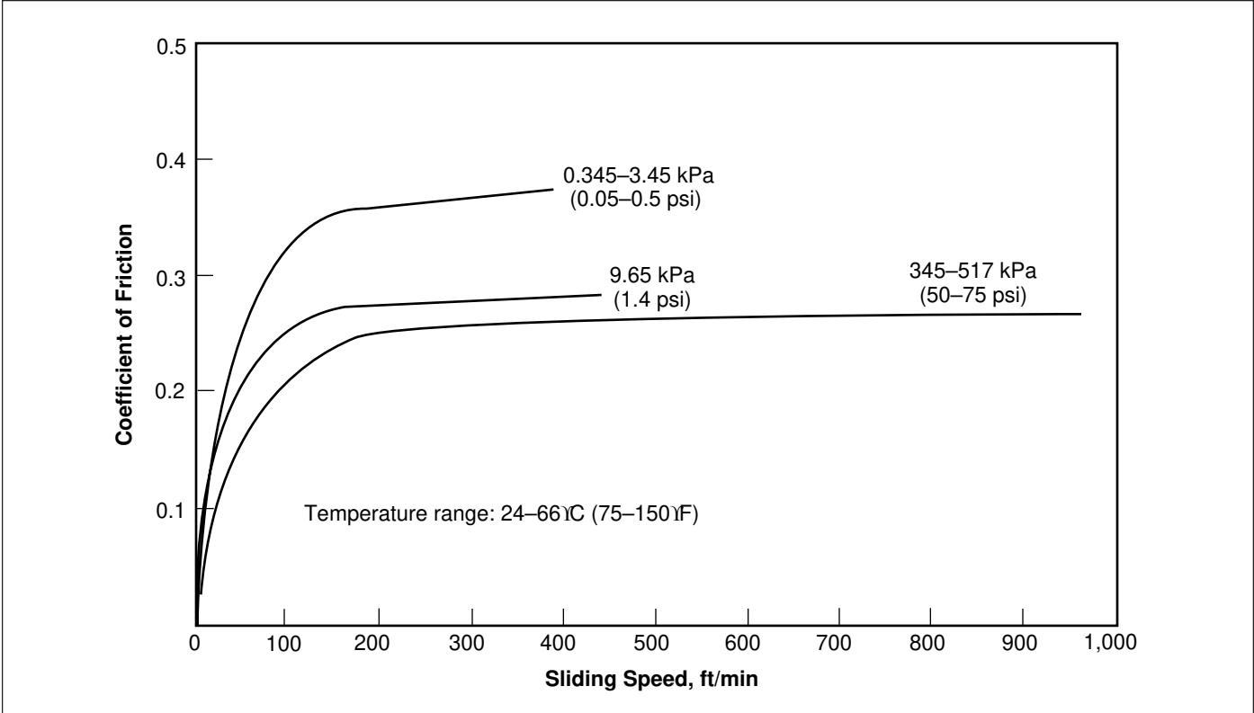
Figure 12. Coefficient of Friction vs. Sliding Speed
