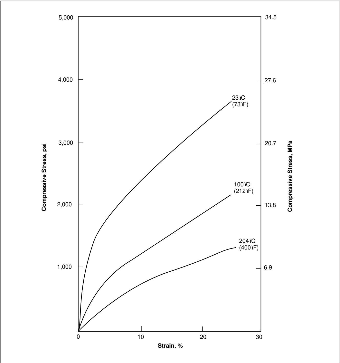
Figure 4. Stress vs. Strain in Compression (ASTM D695)
