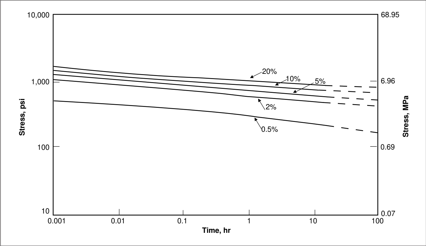
Figure 10a. Tensile Strength Relaxation at 23°C (73°F)
