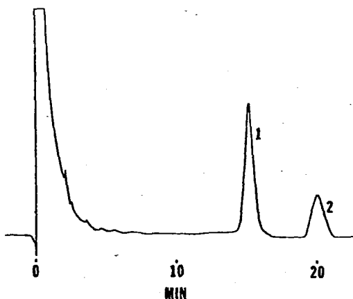
FIG. 1—Electron capture GLC curve from the 0.2 ml \text{SbCl}_5 (Hooker Chemical) perchlorination of 0.50 \mu g Aroclor 1221; 0.51 ng equivalent Aroclor 1221 injected. Peak 1 represents 0.81 ng DCB. Peak 2 represents 0.28 ng BNCB.
