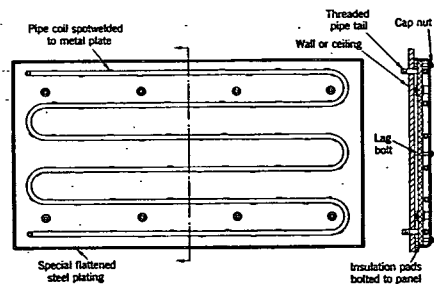
FIG. 5. PILLAR TYPE RADIANT HEAT PANEL
