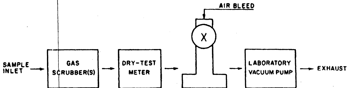
Fig. B8 Sampling Train
