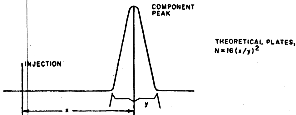
Fig. B9 Calculating Column Efficiency
