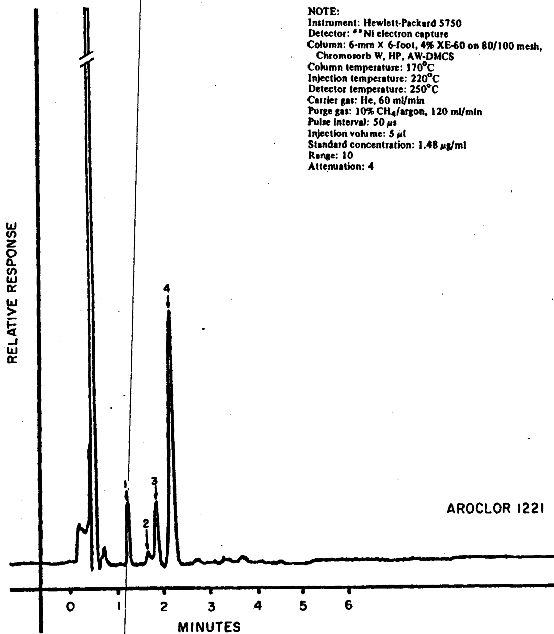
Fig. B3 Aroclor 1221 Electron Capture Chromatogram
