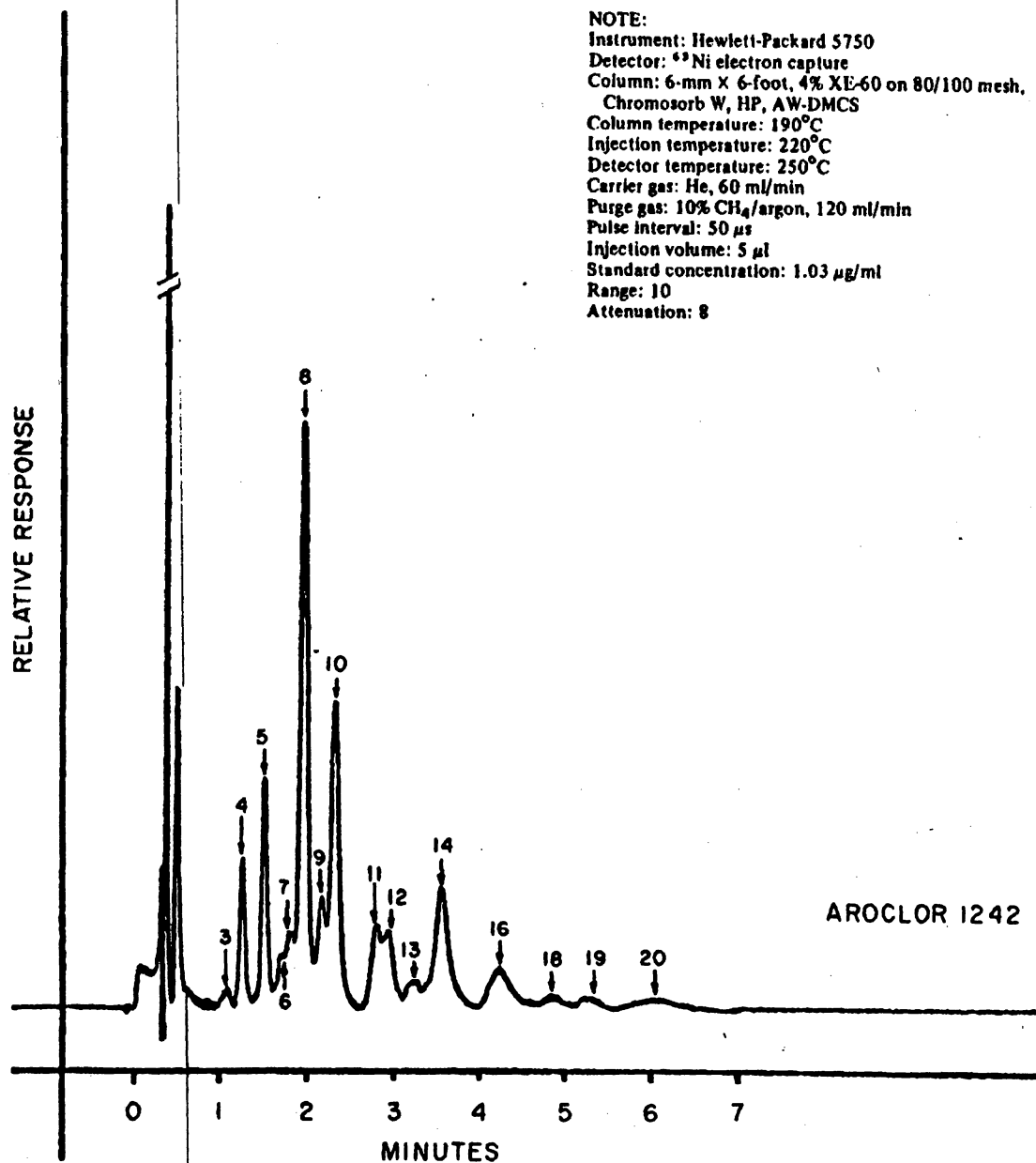
Fig. B4 Aroclor 1242 Electron Capture Chromatogram
