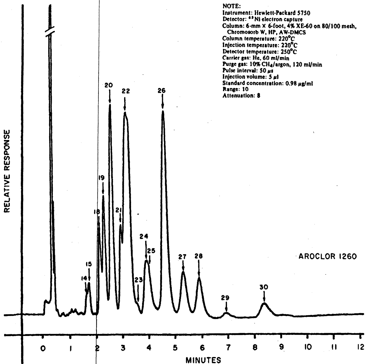
Fig. B7 Aroclor 1260 Electron Capture Chromatogram
