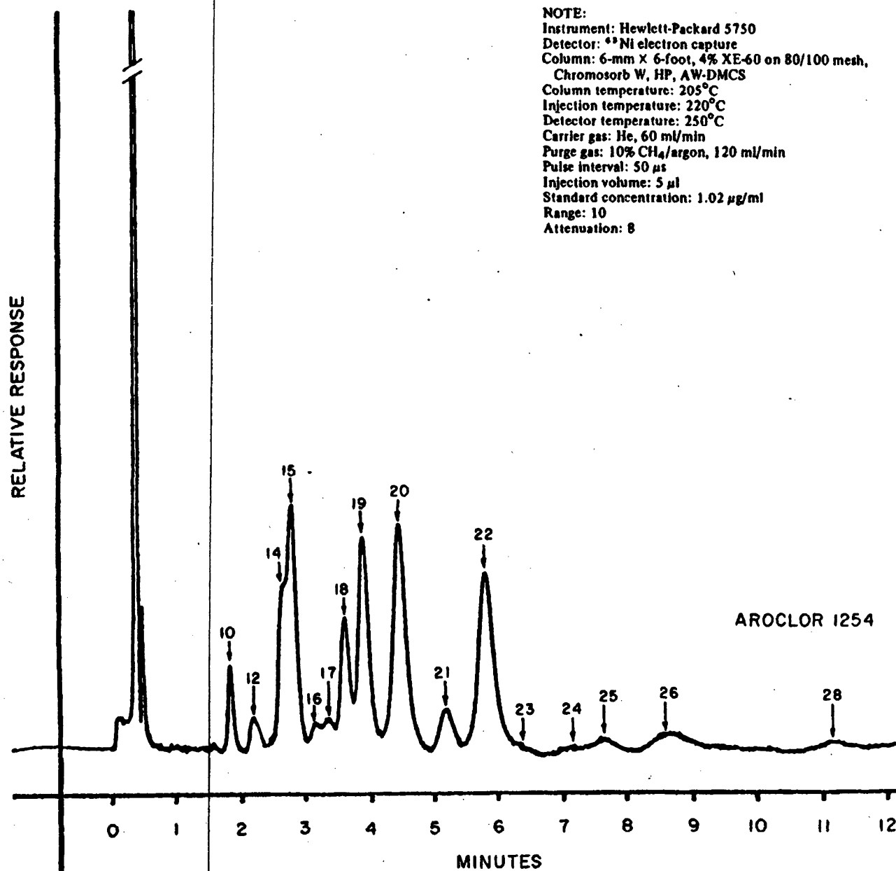
Fig. B6 Aroclor 1254 Electron Capture Chromatogram
