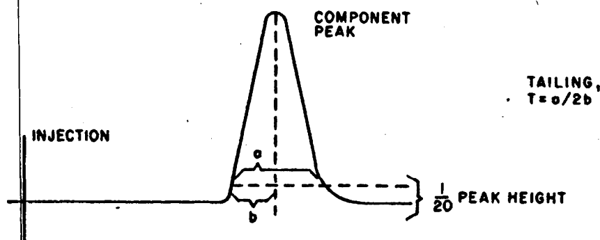
Fig. B10 Calculating the Tailing Factor
