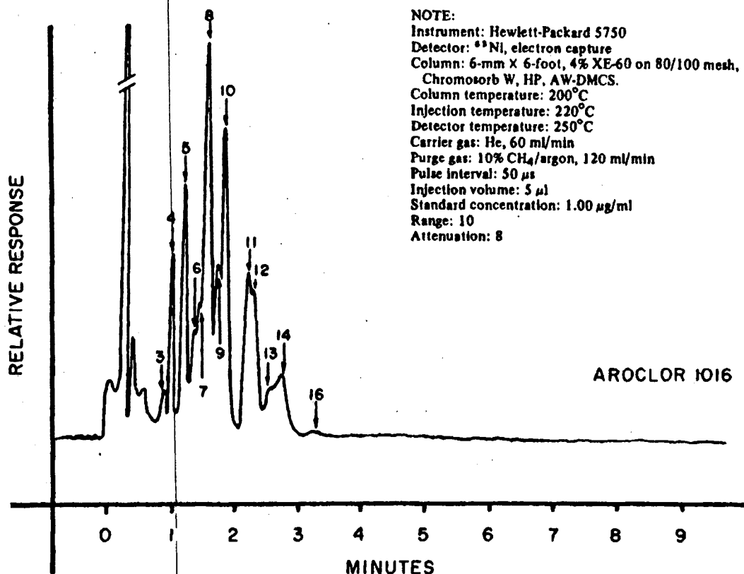
Fig. B1 Aroclor 1016 Electron Capture Chromatogram
