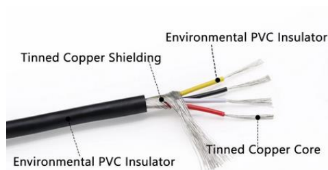
Figure 7 - Example 4-core shielded cable
