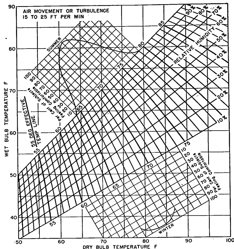
FIG. 10. A.S.H.A.E. COMFORT CHART FOR STILL AIR a,b
