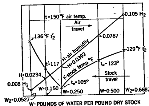
FIG. 7. TEMPERATURE HUMIDITY RELATIONS IN A DRYER
