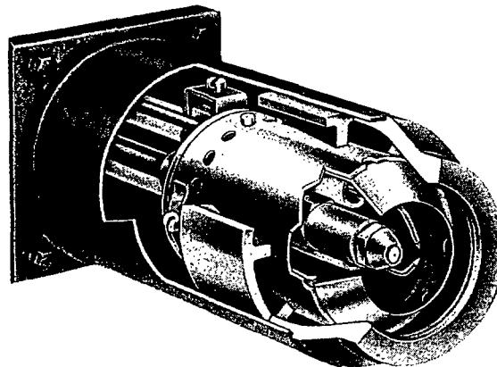
model ES-2 shell head — cutaway view
