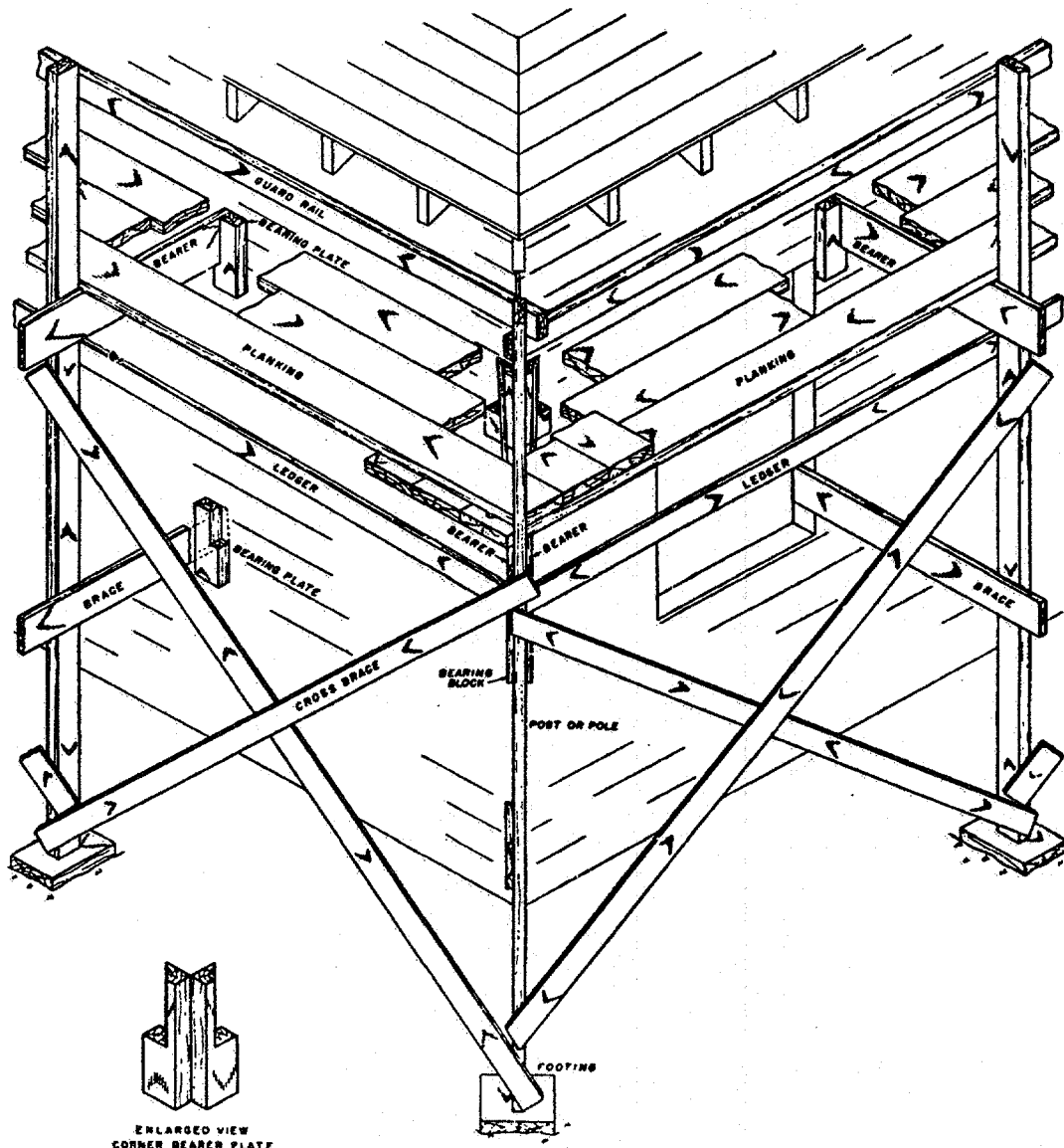
Figure 16. Single Pole Scaffolding-Corner Construction.
