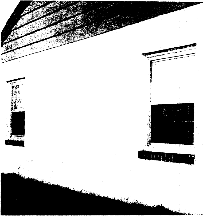
Figure 84. Loss of Adhesion from Chalked Paint.
