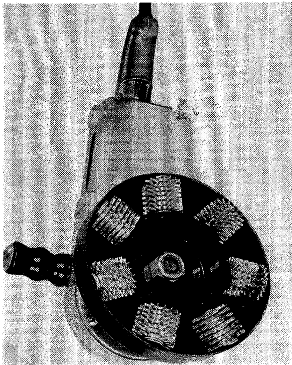
Figure 35. Typical Power Grinding Tool.
