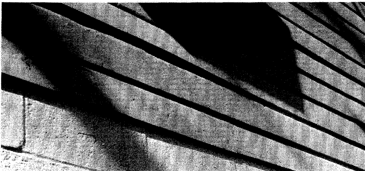
Figure 101. Temperature Blistering.
