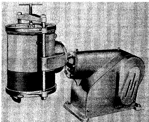
Figure 31. Paint Mixer-Vibrating Shaker.
