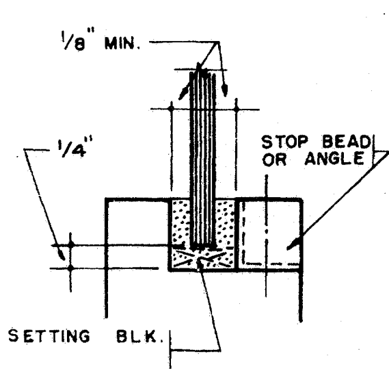
Channel Glazing
