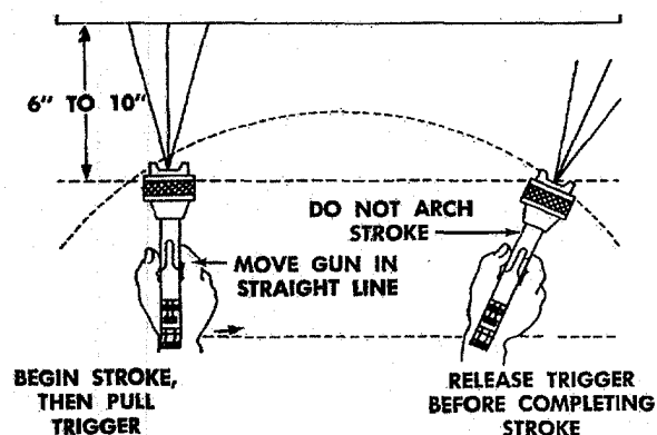
Figure 68. Proper Spray-Gun Stroke.
