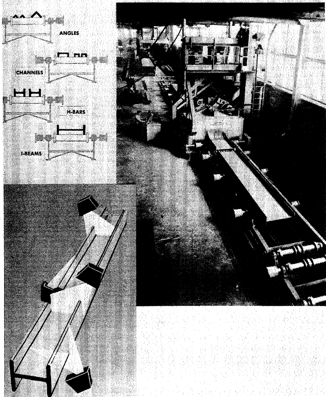
Figure 48. Centrifugal Blasting.
