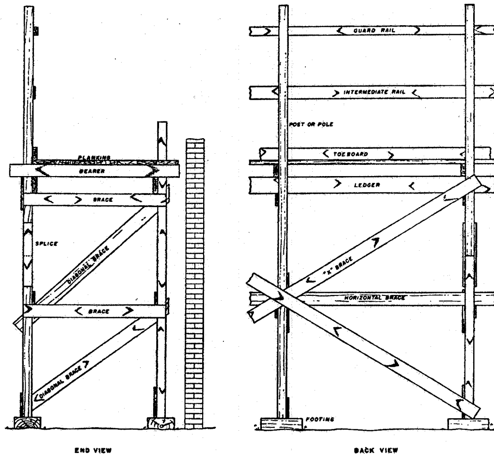
Figure 15. Diagonal Bracing on Double Pole Scaffolding.
