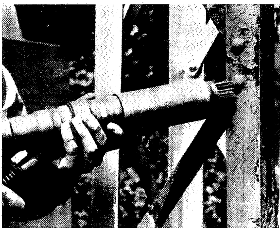
Figure 40. Needle Scaler.
