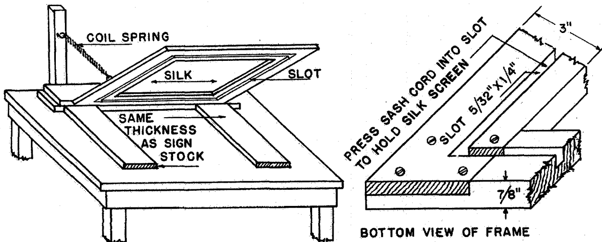
Figure 123. Screen Printing Setup.
