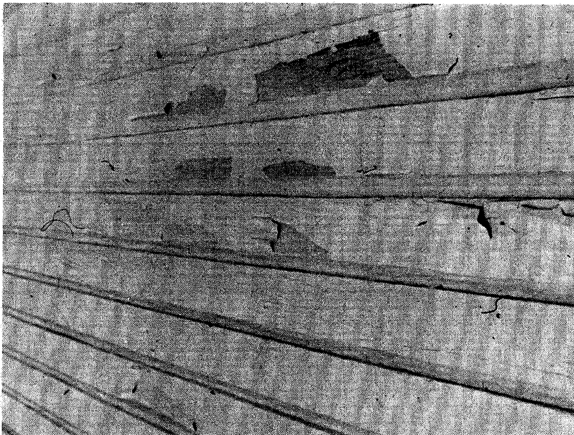
Figure 108. Loss of Adhesion from Moisture.
