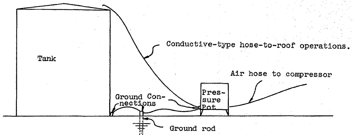
Figure 26. Grounding of Tank and Equipment.
