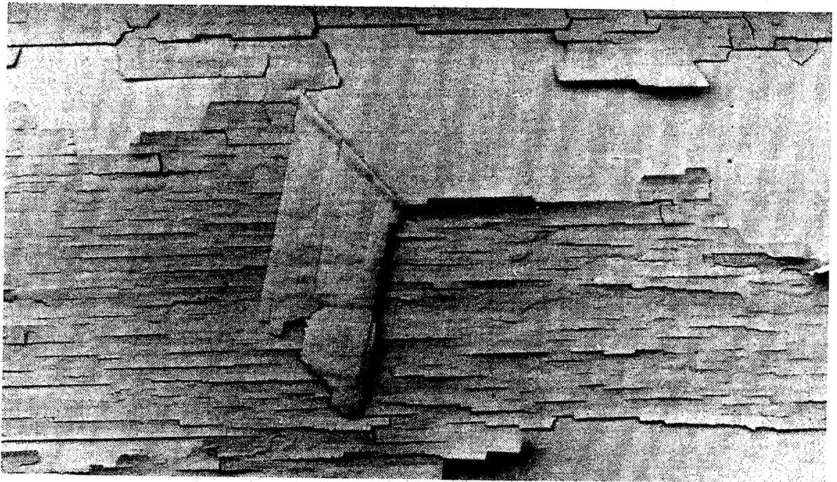
Figure 104. Intercoat Peeling.
