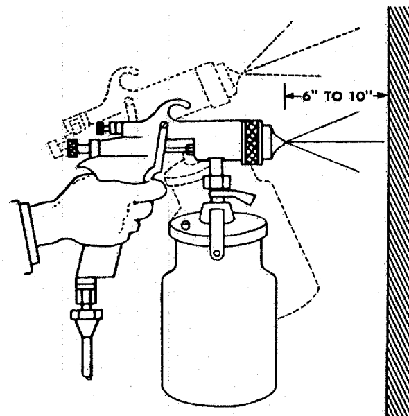
Figure 67. Spray Gun Held Perpendicular to Surface to Prevent Uneven Deposit of Paint.
