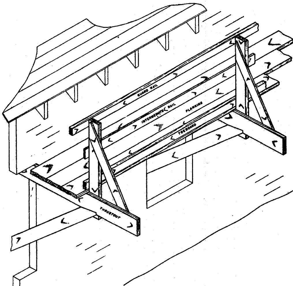
Figure 18. Outrigger Scaffold with Guard Rail.
