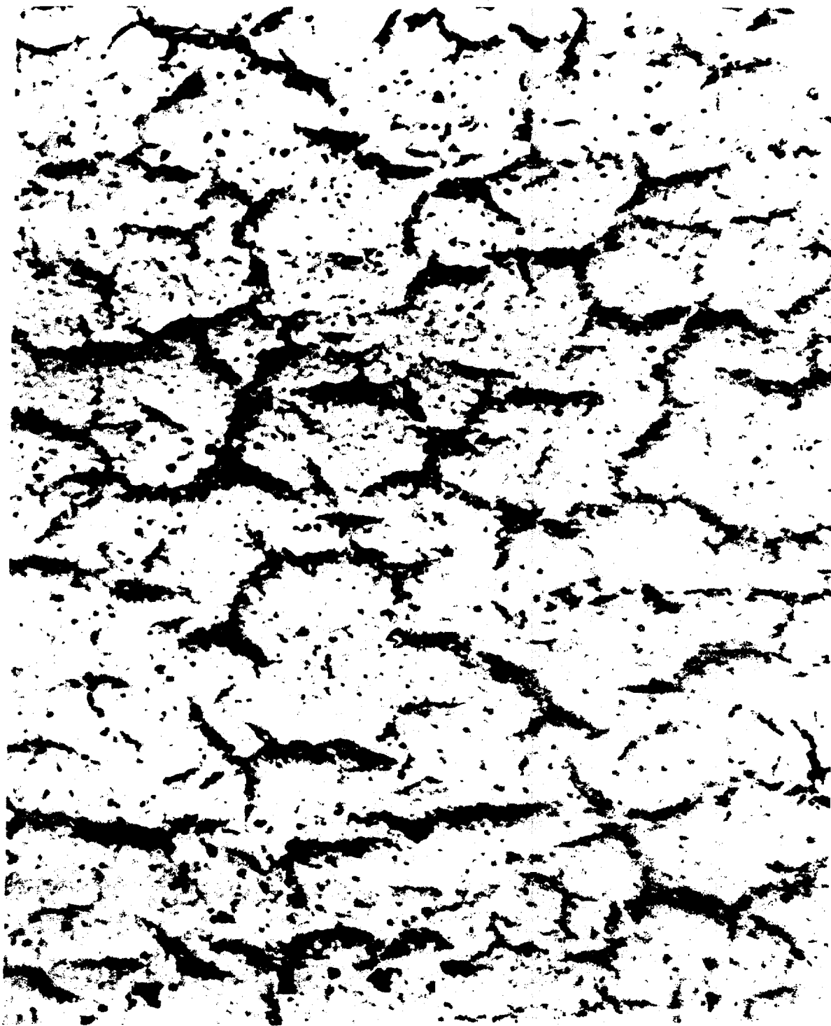
Figure 102. Alligatoring.
