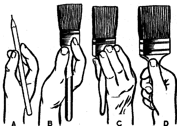
A, B. Grasping brush with pencil grip. C. Grip used for painting walls and floors. D. Simple grip with all fingers around brush handle, suitable for use when painting ceilings.
