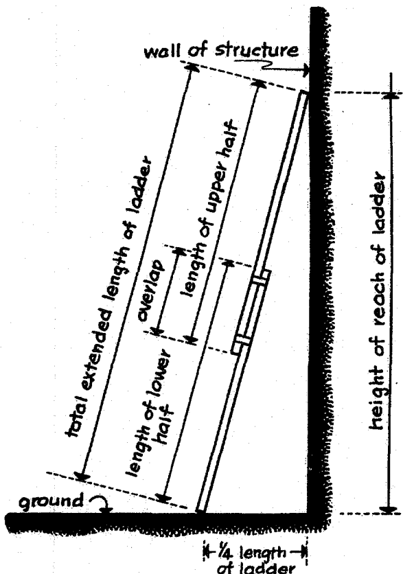
Figure 13. Ladder Stability.
