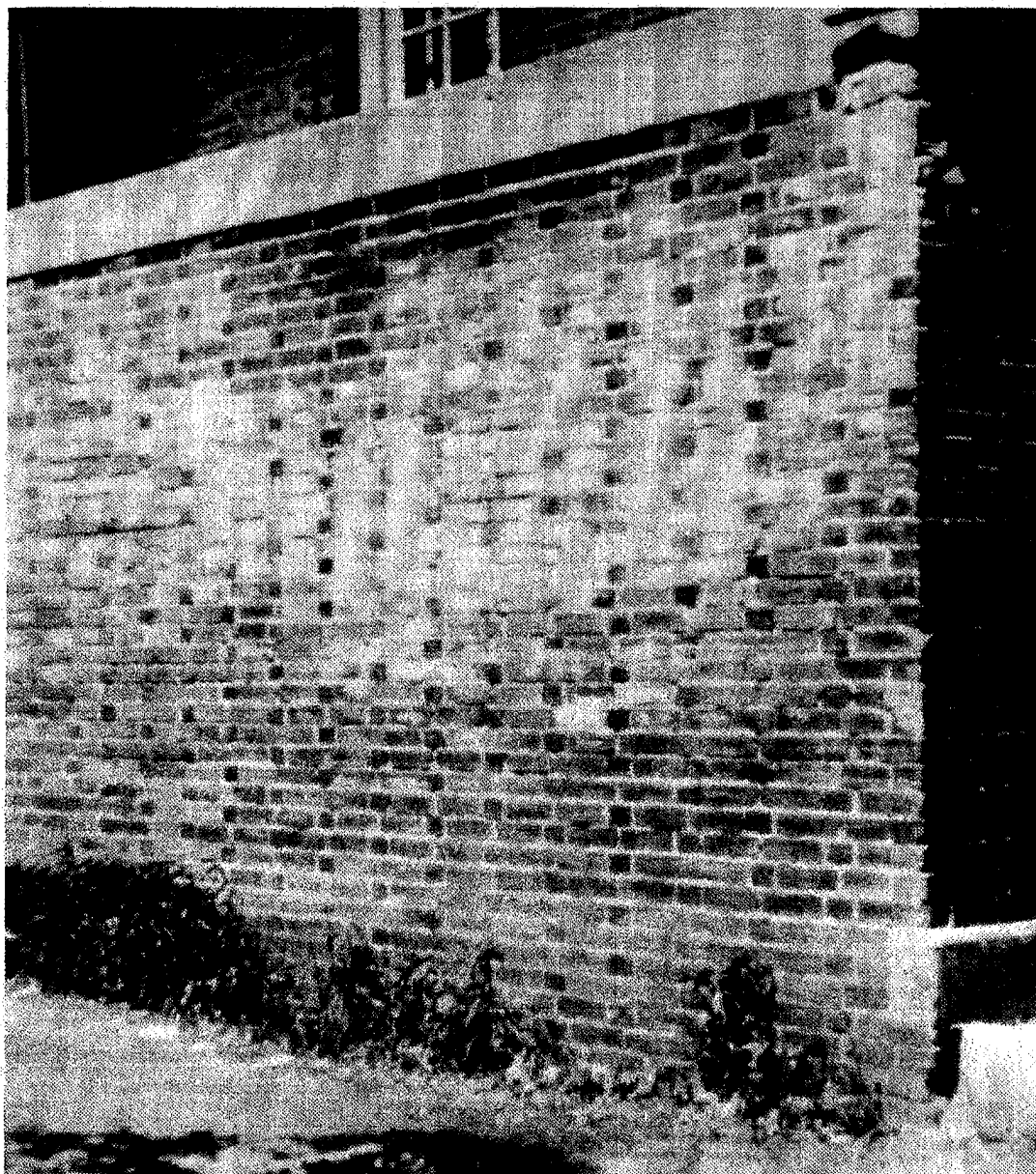
Figure 97. Severe Efflorescence on Brick Wall.
