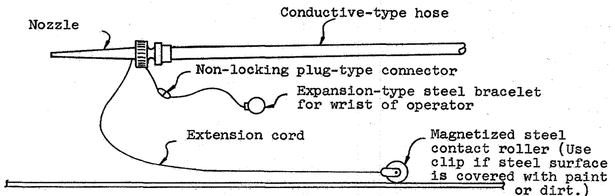
Figure 27. Grounding of Blast Nozzle.
