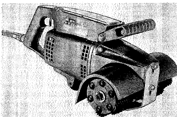
Figure 39. Rotary Impact Cleaning Tool.
