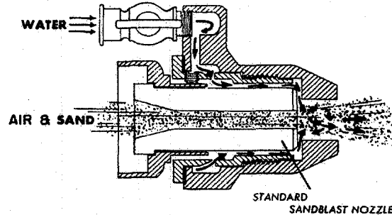
Cross section view of wet blast attachment which sucks water from any water supply for wet blast cleaning.
