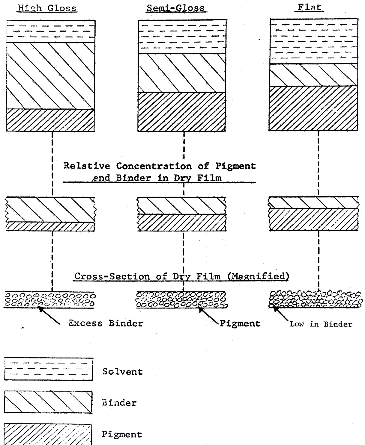
Figure 114. Effect of Pigment/Binder on Gloss.
