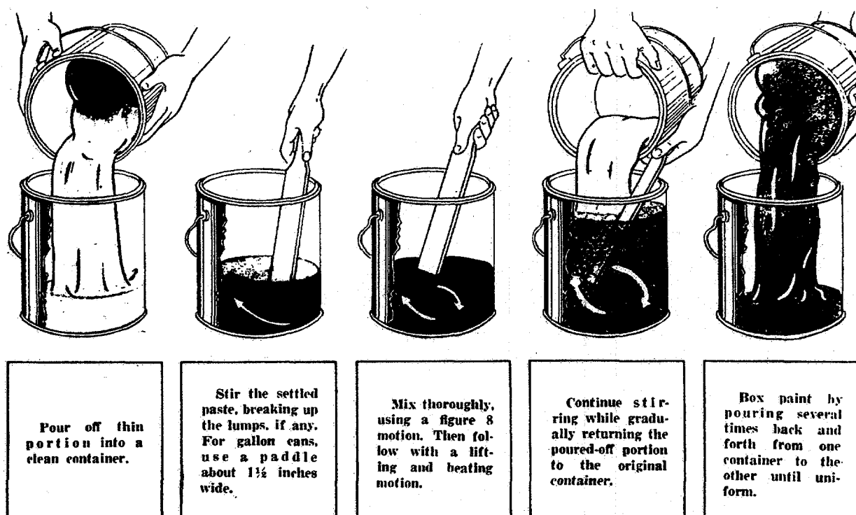
Figure 33. Manual Mixing and Boxing.
