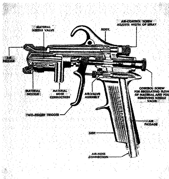
Figure 66. Spray Gun — Cross-Section.
