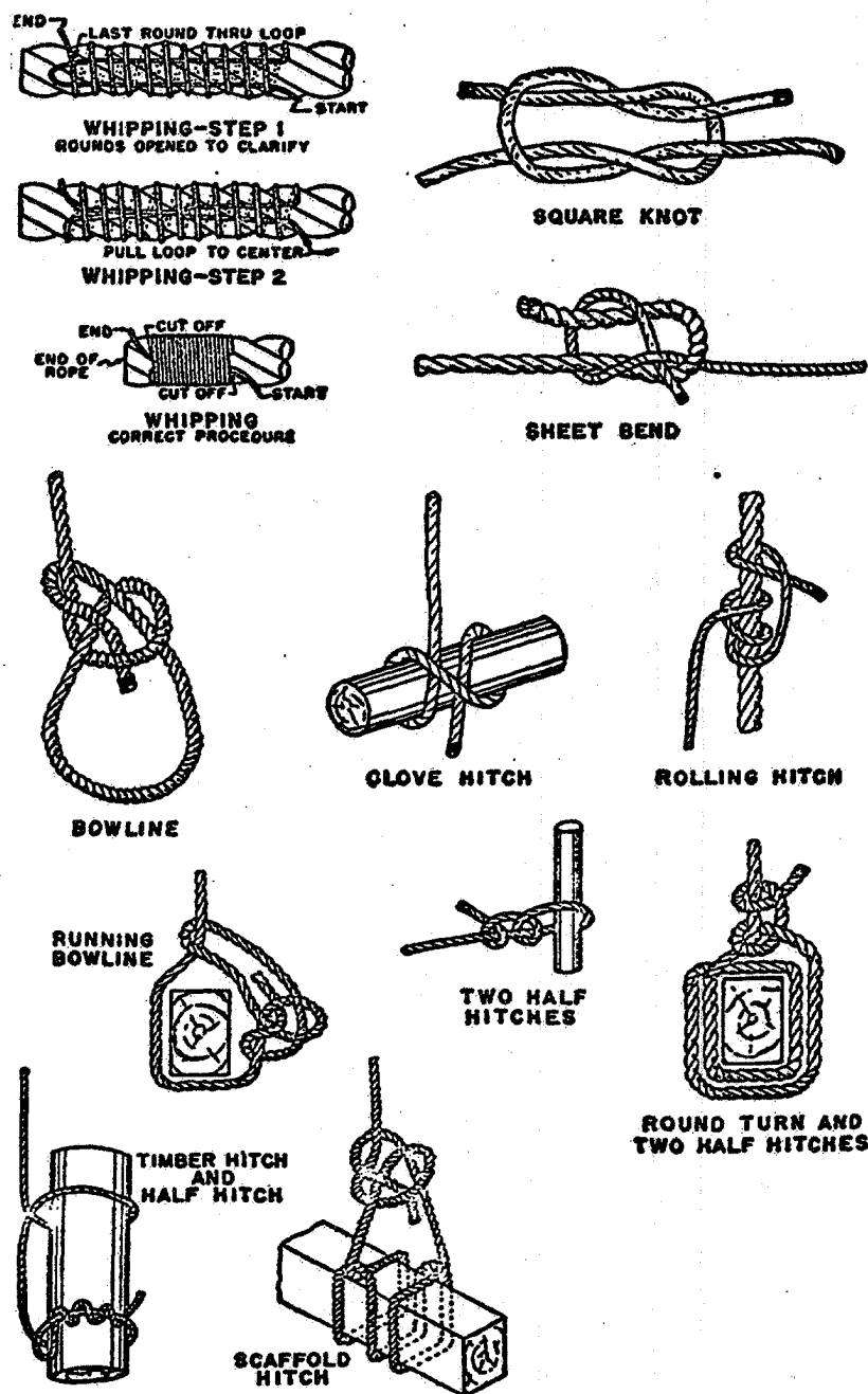
Figure 25. Knots and Hitches Used in Painting Operations.
