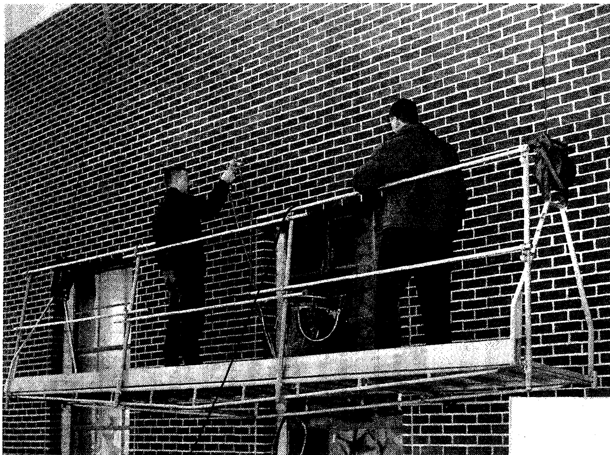
Figure 22. Swinging Scaffold Ladder Platform Type.
