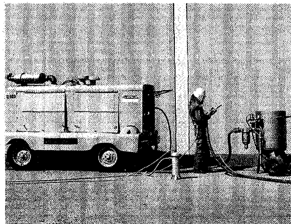
Figure 43. Dry Blast Cleaning Setup.
