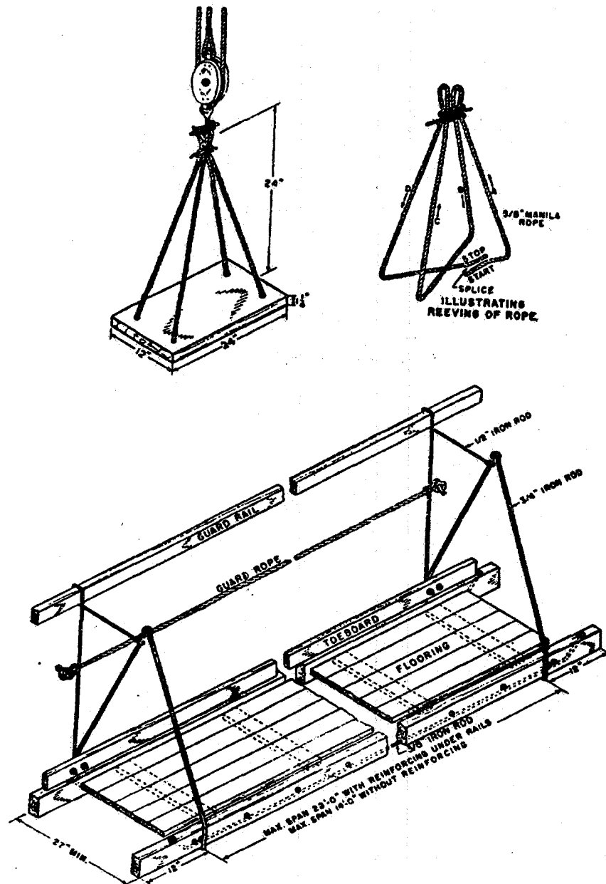
Figure 24. Bosun Chair and Swinging Scaffold (Construction Details).
