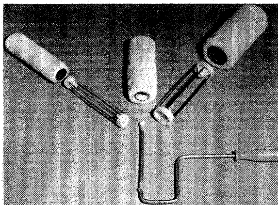
Figure 58. Parts of a Roller.
