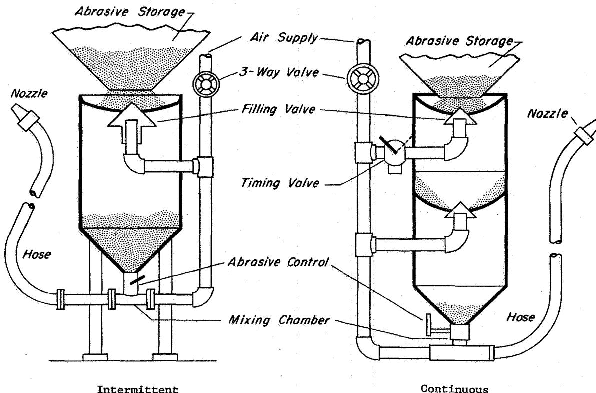
Figure 44. Direct Pressure Blast Cleaning Tanks.
