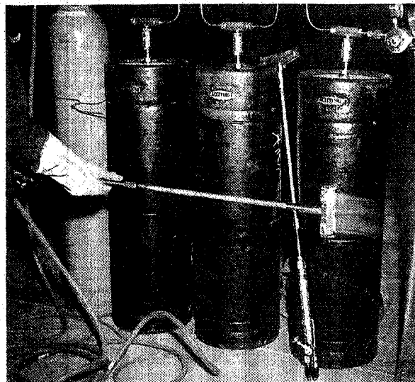
Figure 41. Flame Cleaning Equipment.
