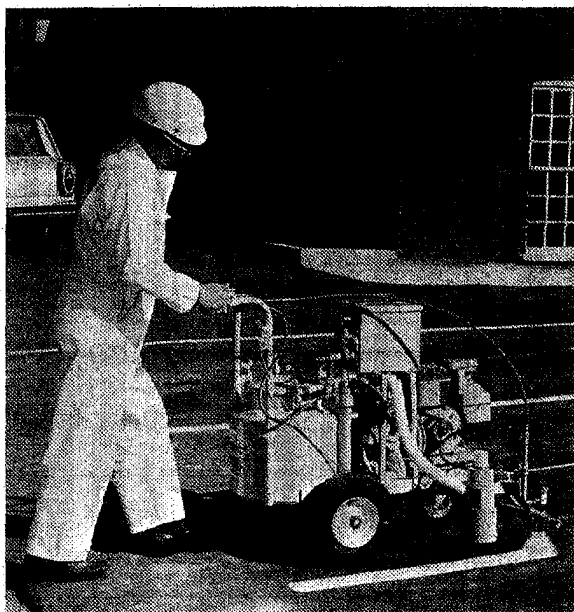
Figure 126. Hand Propelled Traffic Marker.
