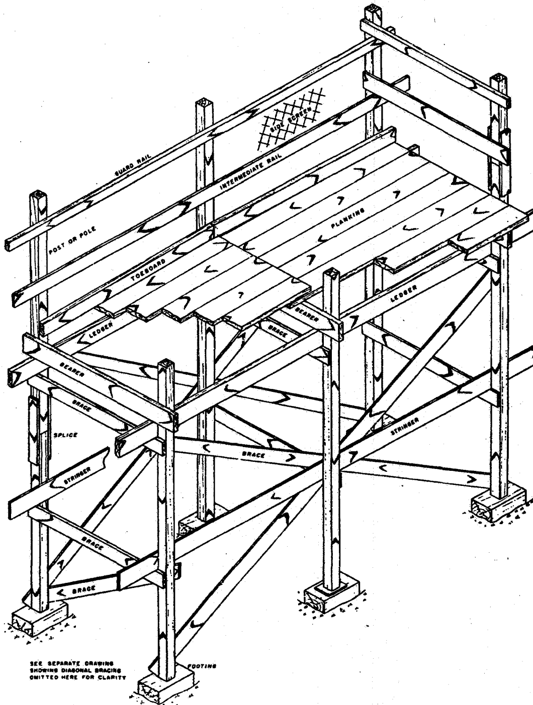
Figure 14. Double Pole or Independent Scaffolding.
