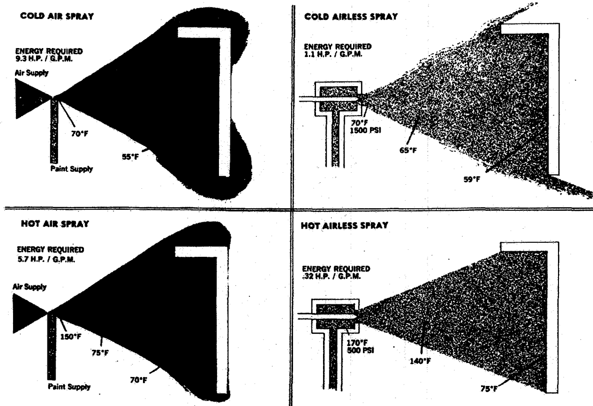
Figure 63. Basic Types of Spray.
