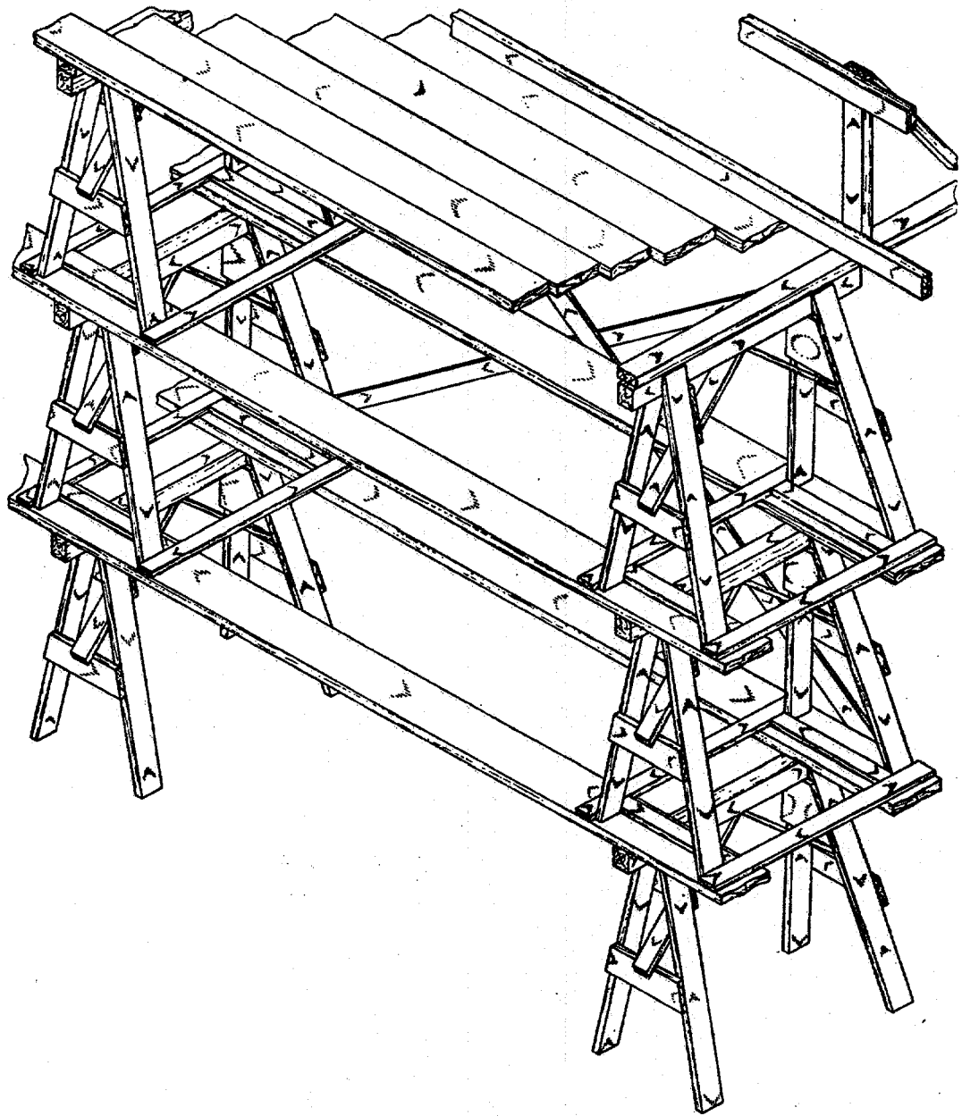
Figure 17. Horse Scaffold, Three Tiers (Max. Height 15 Ft.)
