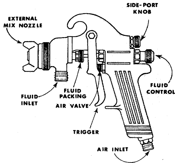
Figure 65. Modern Production Spray Gun.
