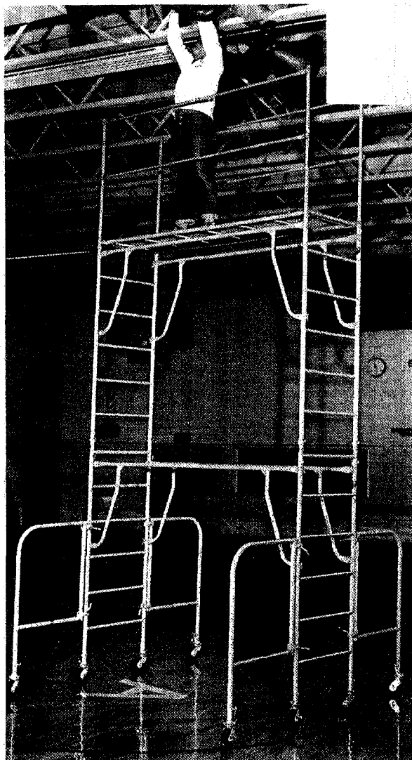
Figure 20. Pipe Scaffolding Roller Outrigger Type.
