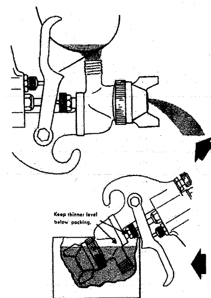
Figure 74. Spray Gun Adjustments and Cleaning.
