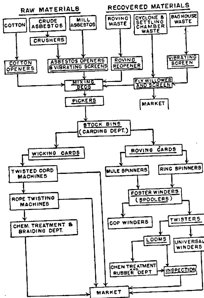
FIGURE 1.—Process flow sheet, asbestos textile plant.
