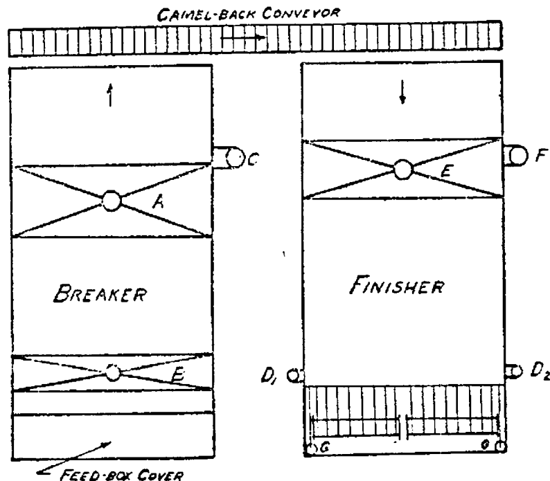
FIGURE 7 — Schematic plot of card exhaust system
