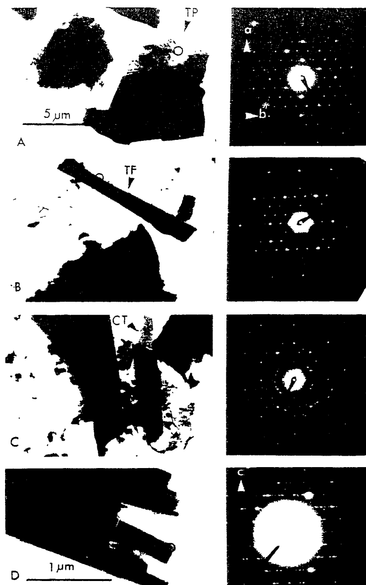
FIGURE 5. Transmission electron micrographs and accompanying selected area electron diffraction (SAED) patterns for cosmetic talc samples. The talc plate (TP) in (A) shows typical polygonal cleavage and diffraction contrast contours for the mineral species. The accompanying SAED pattern displays the characteristic reciprocal ab^* plane pseudo-hexagonal symmetry for talc. Talc a^* and b^* directions indicated on (A). Measurement of pattern indicates a 5.3 Å repeat along a^* and a 9.1 Å repeat for b^* (measured at [110] ). Talc fiber (TF) in (B) displays irregular ends and nonrectilinear edges. The SAED pattern is also pseudo-hexagonal, but some reflection intensities [e.g., the (060), (0.12.0)] are more pronounced. This may be due to both orientation and structural effects. The curled talc plate (CT) in (C) displays an incipient Debye-Scherrer ring pattern (the effects of both folding over of talc and small associated grains). The amphibole fiber (D) was diffracted only on one of the protruding unit forms. The c^* axis is shown, with repeat measured at 5.3 Å. Areas where diffraction patterns were obtained are indicated by location circles; particles were photographed at the SAED magnification \times 26,500 . Scale is the same in A-C, scale in D as marked. Micrographs obtained on a JEOL JEM 120U with an accelerating voltage at 120 kV.
