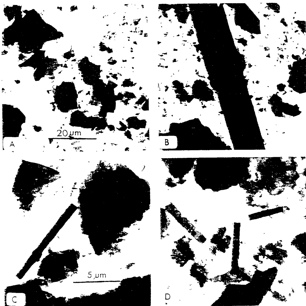
FIGURE 4. Transmission electron micrographs of cosmetic talc samples composed primarily of plates, with an occasional large talc fiber (B, C), talc with many talc fibers (D). Scale is the same in (A) and (B) and in (C) and (D). All selected area electron diffraction patterns obtained on fibers (also those consistent on the plates) (see Fig. 5, A and B). In all talc-containing samples examined by electron microscopy, talc grains tended to range from 25 to 0.2 \mu\text{m} in greatest dimension. Micrograph obtained on a JEOL JEM 100 U with an acceleration voltage of 120 kV.
