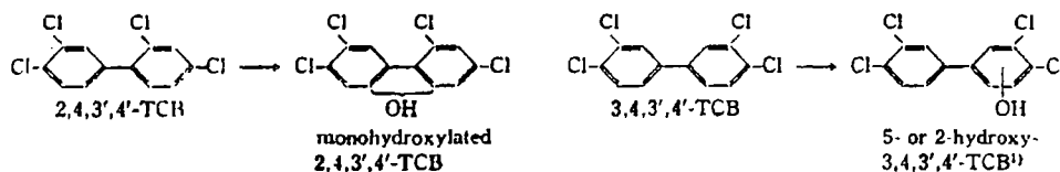
Fig. 5. Biotransformation of 2,4,3',4'- and 3,4,3',4'-TCB in the Rat
