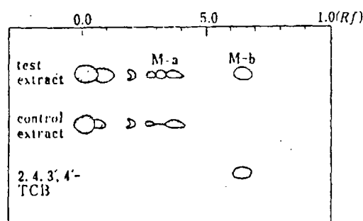
Fig. 1. Thin-Layer Chromatogram of Extract of the Third Day Feces and 2,4,3',4'-TCB
