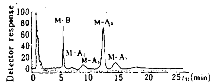
Fig. 2-B. Gas Chromatogram of Trimethylsilylated Extract of the Third Day Feces
