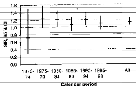
Figure 2. Incidence of lung cancer (International Classification of Diseases, 7th revision-162.1) by calendar period among Swedish construction workers heavily exposed to asbestos. (SIR = standardized incidence ratio, 95% CI = 95% confidence interval)
