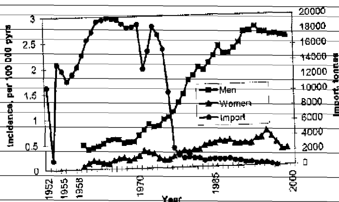
Figure 1. Annual import of asbestos in Sweden and age-standardized incidence of tumors of the pleura (International Classification of Diseases, 7th revision =162.2) by gender. (pyrs = person-years)
