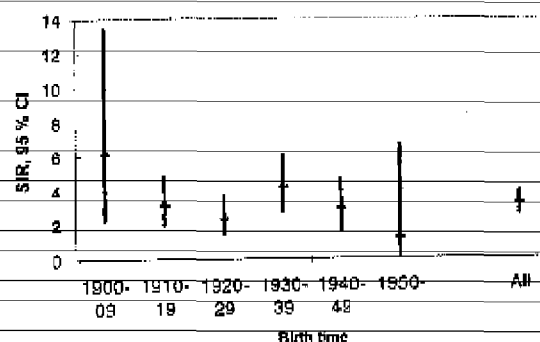
Figure 3. Incidence of pleural tumors (International Classification of Diseases, 7th revision-162.2) by time of birth among Swedish construction workers heavily exposed to asbestos. (SIR = standardized incidence ratio, 95% CI = 95% confidence interval)
