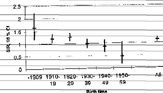
Figure 4. Incidence of lung cancer (International Classification of Diseases, 7th revision-162.1) by time of birth among Swedish construction workers heavily exposed to asbestos. (SIR = standardized incidence ratio, 95% CI = 95% confidence interval)
