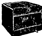
Model BAV Residential Evaporator with two drain pans for mounting in "A" position above furnace or in "V" position below counter-flow furnace. Available in 2, 3, 4, 5 and 7½ ton capacities.
