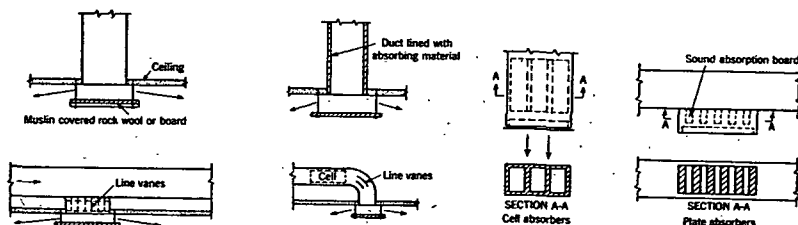
FIG. 2. OUTLET CELLS FOR PAN OUTLETS OR GRILLES
