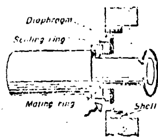
4 Stationary seal
