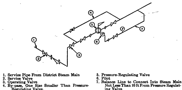
FIG. 2. PRESSURE-REGULATING VALVE WITH BYPASS FOR LOW PRESSURE SERVICE
