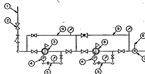
FIG. 3. TWO-STAGE PRESSURE-REDUCING AND PRESSURE-REGULATING EQUIPMENT (Used Where High-Pressure Steam is Supplied for Low-Pressure Requirements).
