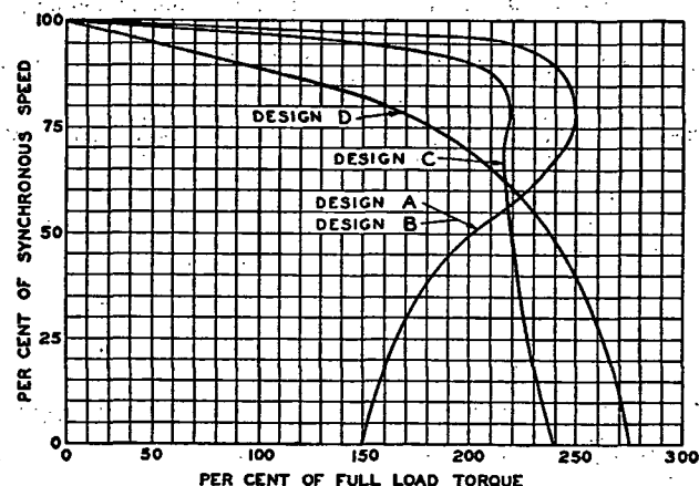
FIG. 1. SPEED TORQUE CHARACTERISTICS OF SQUIRREL-CAGE MOTORS
