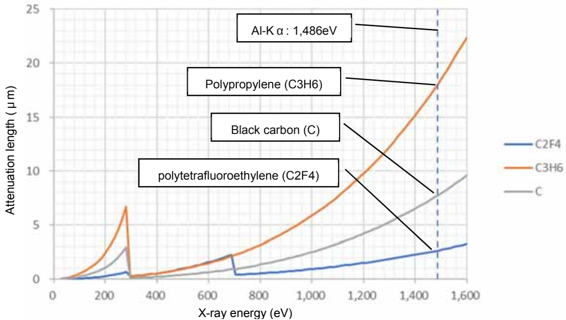
Figure 33 X-ray attenuation lengths from Aluminum 3
