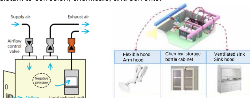
Figure 56 Example of air volume control in a chemical/ Other exhaust applications
