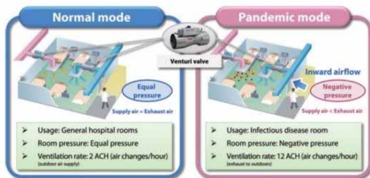
Figure 57 Image of negative and positive pressure control in a hospital room
