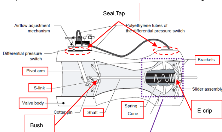
Figure 58 Valve image
