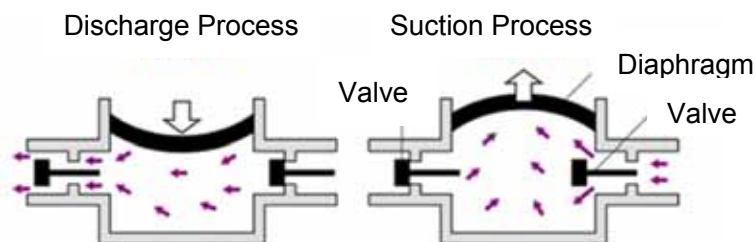
Figure 23 Explanation on Pumps 2
