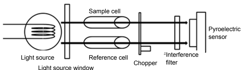
Figure 47 Oil content analyzer bench structure
