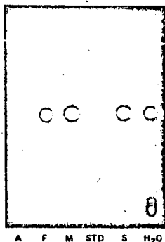
Fig. 2D. Radioautogram of TLC plate containing extracts of water and organisms treated with DDE. A (alga), F (fish), M (mosquito larva), S (snail) and STD ( 14 C-radiolabeled compound).
