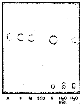
Fig. 2C. Radioautogram of TLC plate containing extracts of water and organisms treated with 2,4,5,2',5'-pentachlorobiphenyl. A (alga), F (fish), M (mosquito larva), S (snail) and STD ( 14 C-radiolabeled compound).
