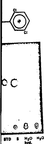
Figure 2C. Radioautogram of TLC plate containing extracts of water and organisms treated with 2,4,5,2',5'-pentachlorobiphenyl. A (alga), F (fish), M (mosquito larva), S (snail) and STD ( 14 C-radiolabeled compound).
