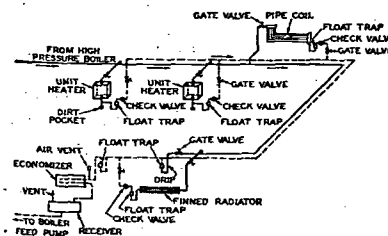
Fig. 9....Typical High-Pressure Heating System
