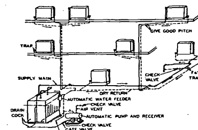
Fig. 10....Typical Installation Using Condensate Pump
