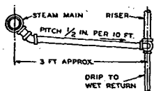
Fig. 5....Typical Steam Runout where Risers are Dripped
