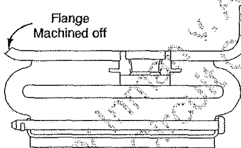
Fig. 14d - Turned Down Flange
