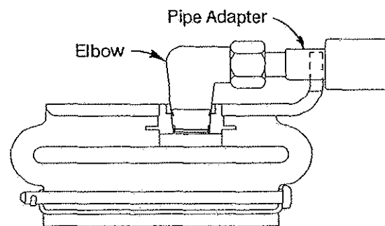
Fig. 15d - Pipe Adapter
