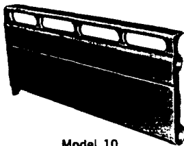
Model 10 Steam Rating per lineal foot 3.4 sq ft
