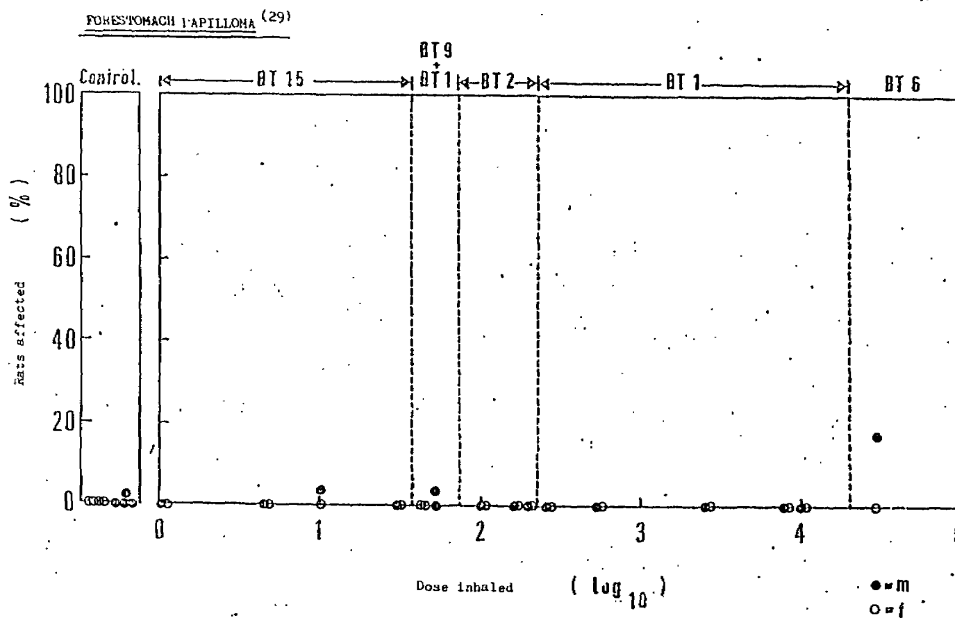
Fig. 12: Proportion of rats affected by forestomach papilloma (29) as a function of the dose
