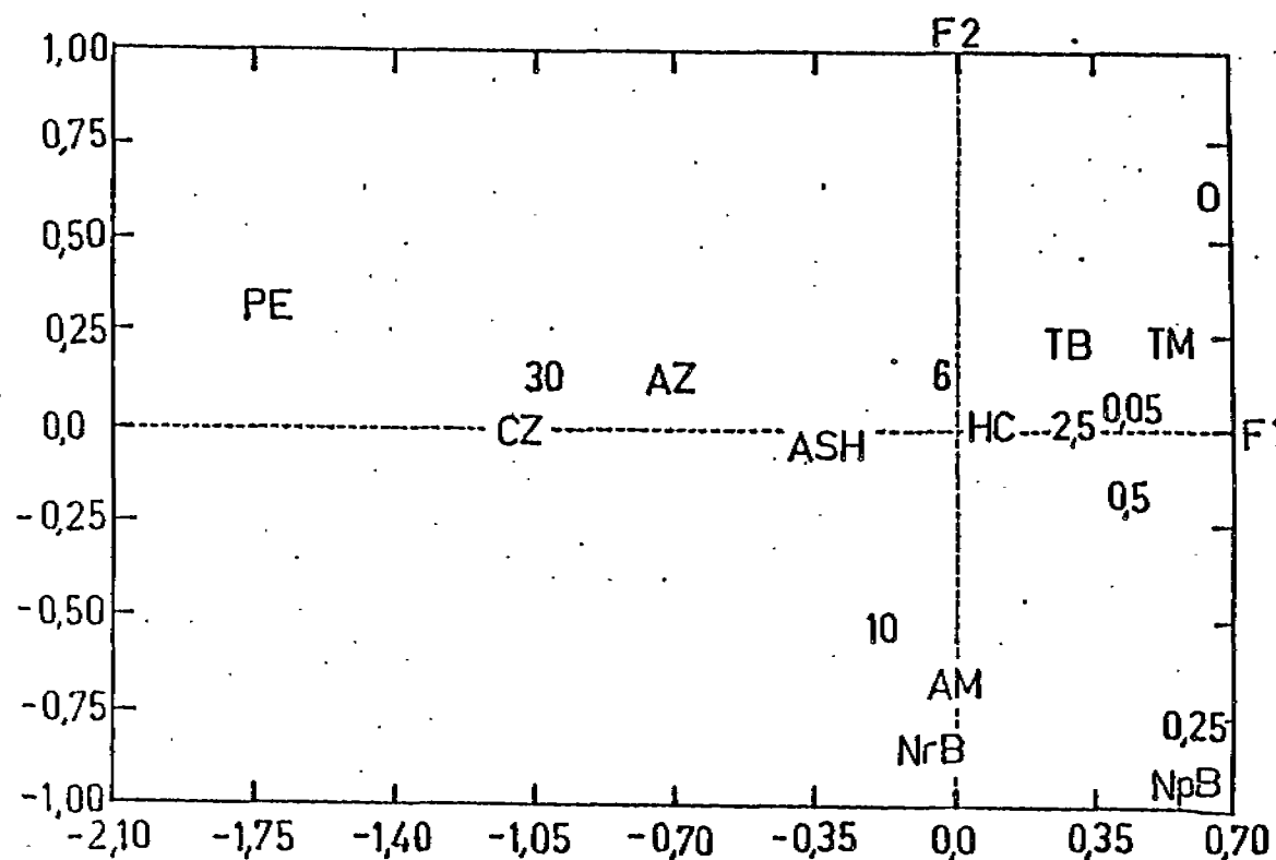
Fig.22: Factorial correspondence analysis (26) between the image points of the doses and the image points of the tumours. AM = mammary adenocarcinoma; ASH = hepatic angiosarcoma; AZ = adenoma of Zymbal gland; CZ = carcinoma of Zymbal gland; HC = hepatocarcinoma; PE = forestomach papilloma; NpB = nephroblastoma; NrB = neuroblastoma, TB = benign tumours, TM = malignant tumours. The doses are expressed in 10 3 ppm, 4 h/d, 5 d/w, for 1 year.
