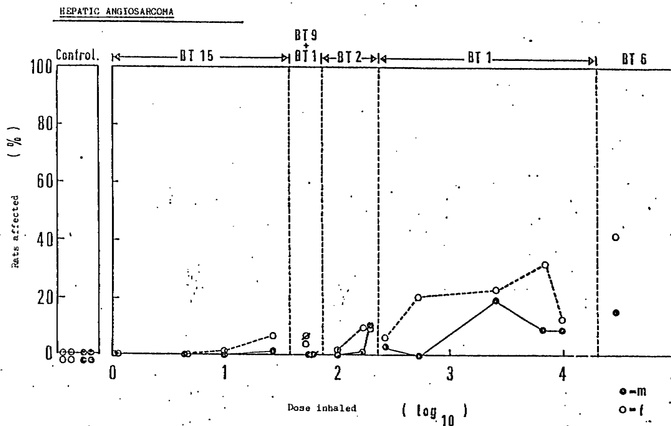
Fig. 5: Proportion of rats affected by hepatic angiosarcoma as a function of the dose
