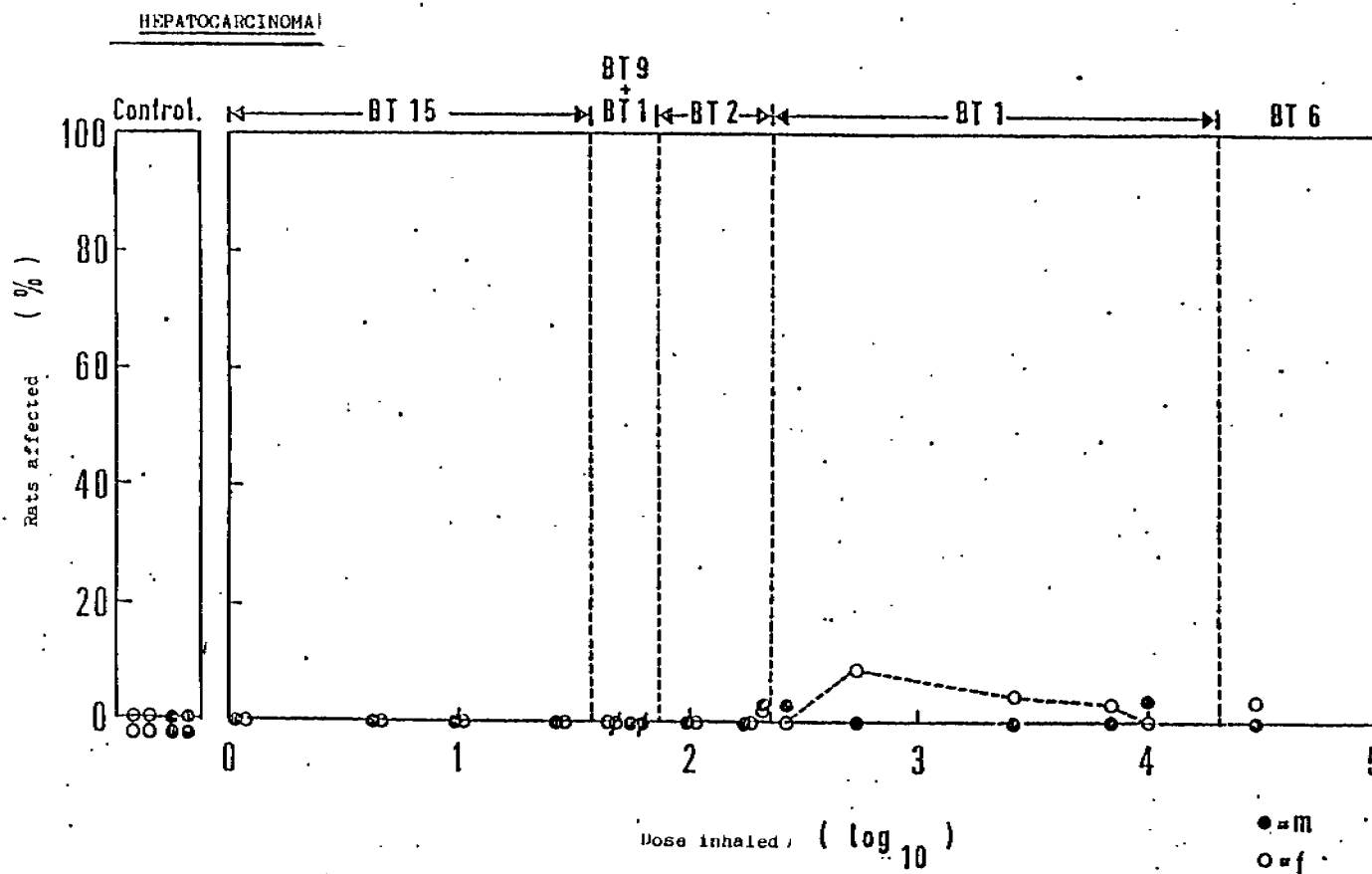
Fig. 13: Proportion of rats affected by hepatocarcinoma as a function of the dose
