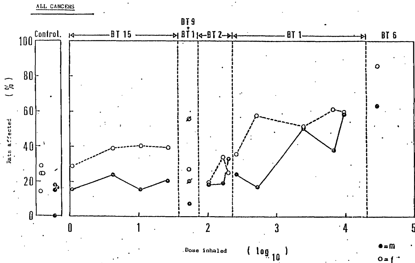
Fig. 14: Proportion of rats affected by all cancers as a function of the dose
