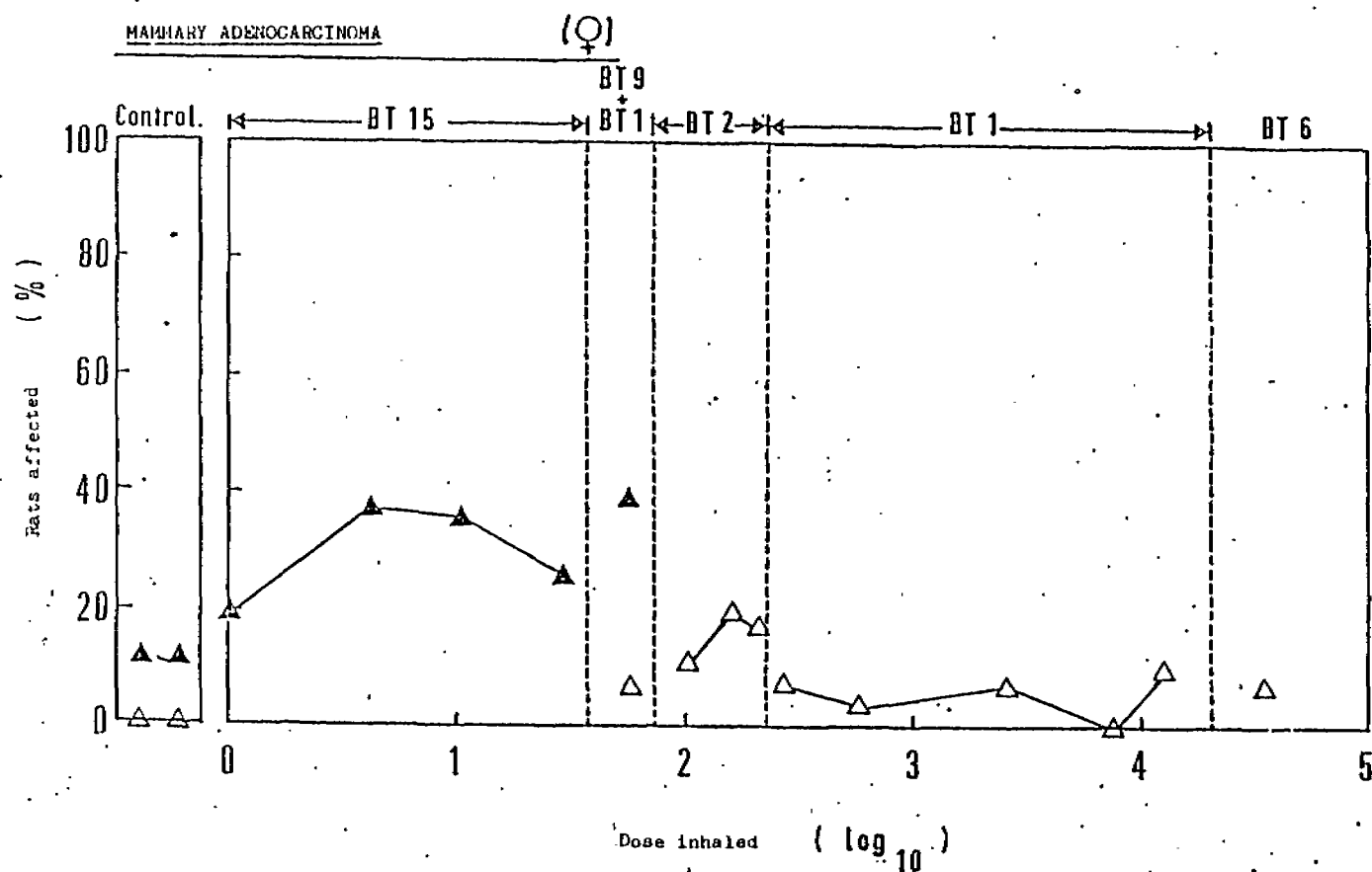
Fig.10: Proportion of rats affected by mammary adenocarcinoma as a function of the dose
