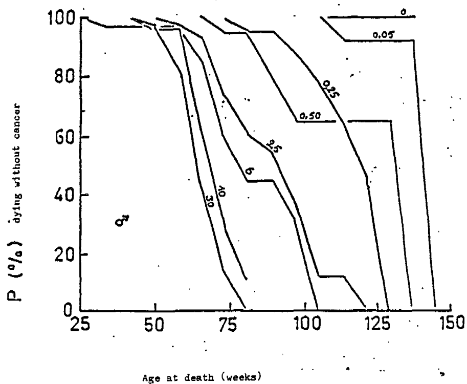
Fig. 15: Actuarial method. Survival without cancer in the Sprague-Dawley rat exposed by inhalation to various doses of VC (expressed in 10^3 ppm, 4 h/d, 5 d/w for 1 year). Maltoni's data.
