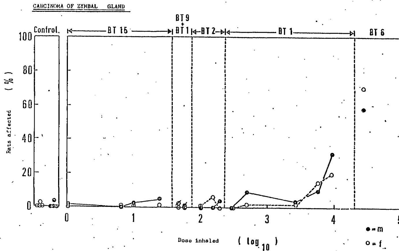
Fig. 7: Proportion of rats affected by cancer of Zymbal gland as a function of the dose
