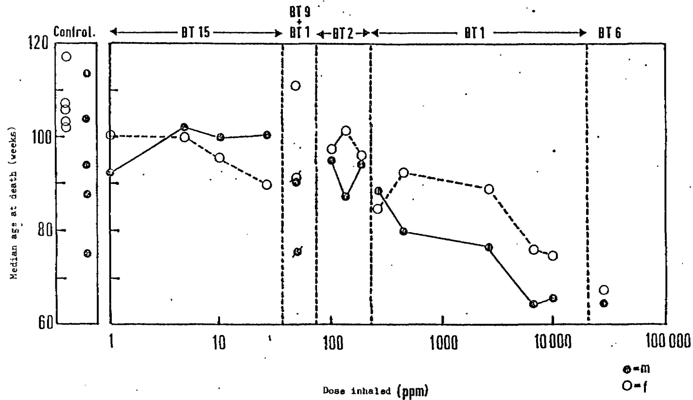
Fig. 12: Reduction in median life of the rats as a function of the dose
