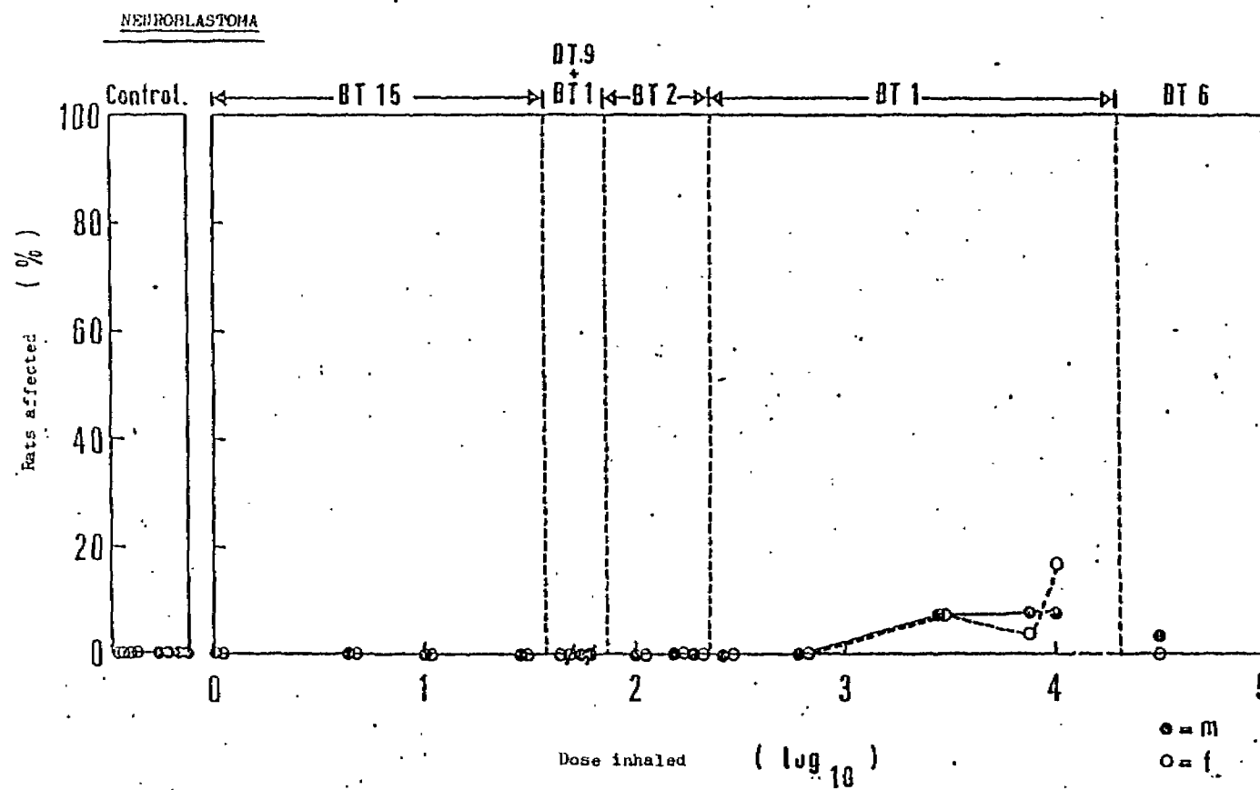
Fig.9: Proportion of rats affected by neuroblastoma as a function of the dose
