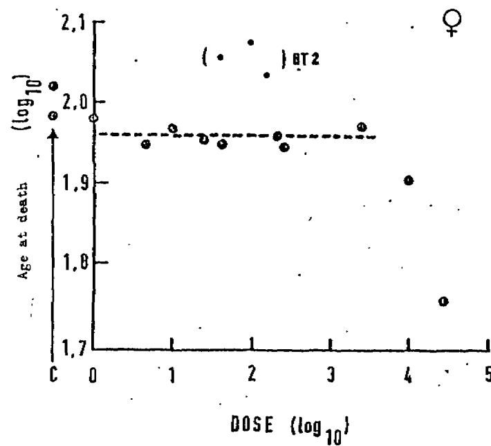
Fig. 11: Female rats with mammary adenocarcinoma: no shortening of life
