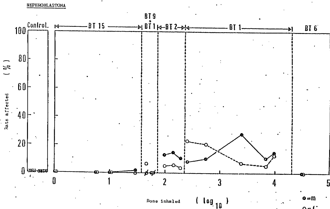
Fig. 8: Proportion of rats affected by nephroblastoma as a function of the dose
