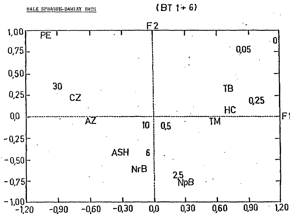
Fig. 21: Factorial correspondence analysis (26) between the image points of the doses and the image points of the tumours. ASH = hepatic angiosarcoma; AZ = adenoma of Zymbal gland; CZ = carcinoma of Zymbal gland; HC = hepatocarcinoma; NpB = nephroblastoma; NrB = neuroblastoma; PE = forestomach papilloma; TB = all other benign tumours; TM = all other malignant tumours. The doses are expressed in 10^5 ppm, 4 h/d, 5 d/w for 1 year.
