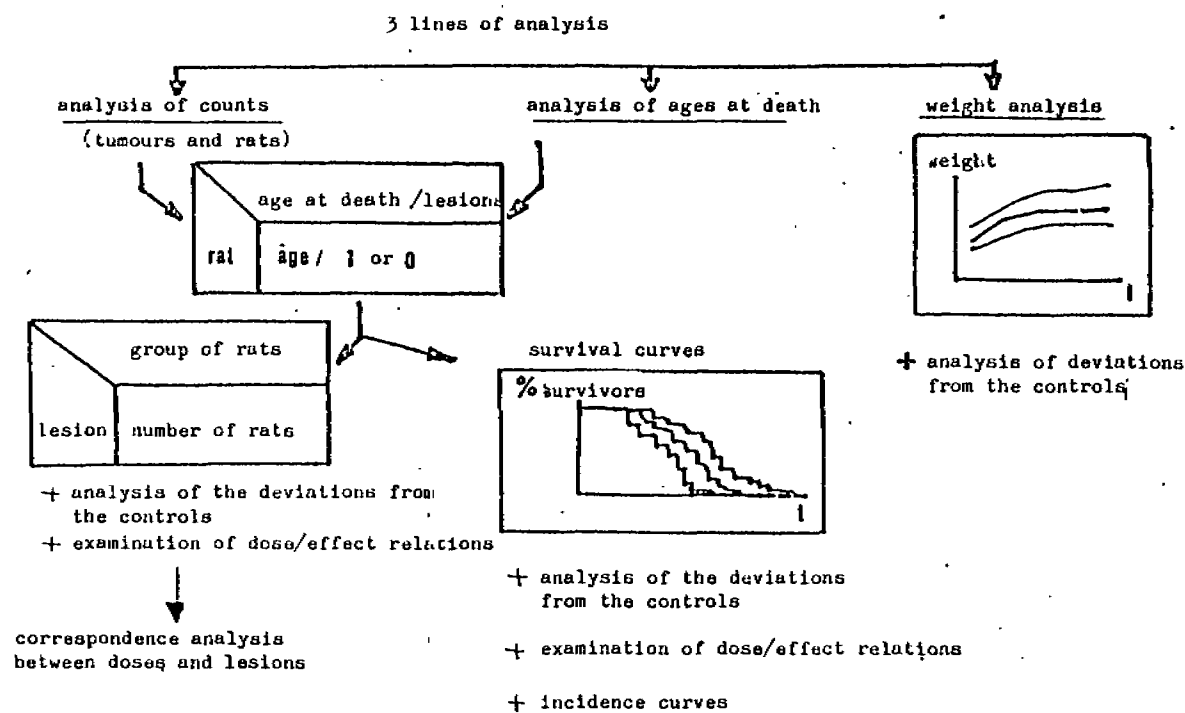
Fig.3: Plan of the statistical analysis (analysis of the data)
