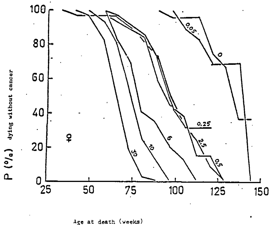
Fig. 16: Actuarial method. Survival without cancer in the female Sprague-Dawley rat exposed by inhalation to various doses of VC (expressed in 10^3 ppm, 4 h/d; 5 d/w for 1 year). Maltoni's data.
