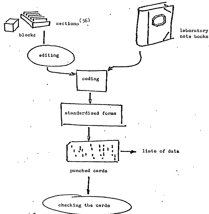
Fig.2: Plan of the statistical analysis (data collection)
