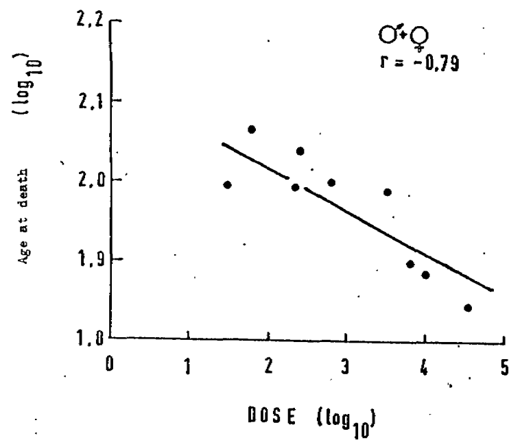
Fig.6: Rats with hepatic angiosarcoma. Reduction in mean survival time
