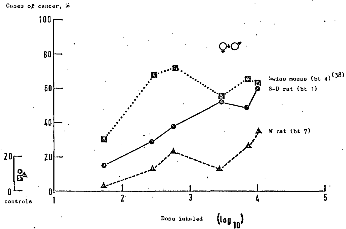
Fig. 26: Interspecies comparison in Prof. Maltoni's studies
