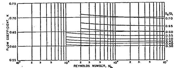
FIG. 8. FLOW COEFFICIENTS, K , FOR SQUARE-EDGED ORIFICE PLATES AND RADIUS TAPS IN SMOOTH PIPE
