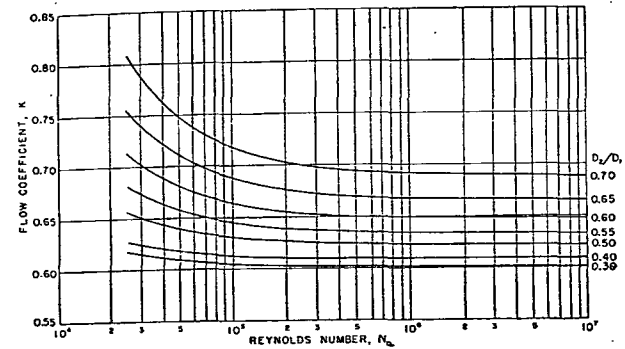
FIG. 7. FLOW COEFFICIENTS, K , FOR SQUARE-EDGED ORIFICE PLATES AND FLANGE TAPS IN SMOOTH PIPE
