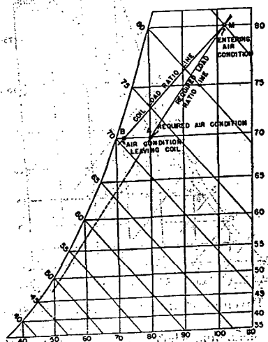
FIG. 14. PSYCHROMETRIC LAYOUT FOR COIL SELECTION USING REHEAT
