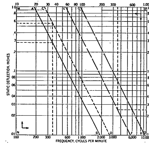
FIG. 11. STATIC DEFLECTION FOR VARIOUS FREQUENCIES
