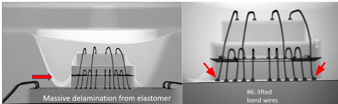
Elastomer delamination and broken wires after decompression test using non fluoroelastomers
