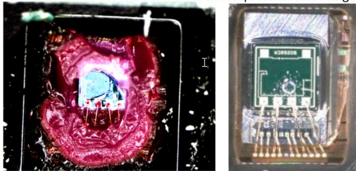
Catastrophic status of elastomer after soapy water exposure in comparison with robust fluoroelastomer
