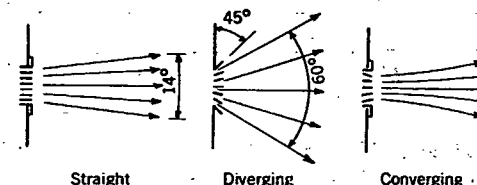
FIG. 4. SPREAD OF AIR STREAM WITH VARIOUS VANES
