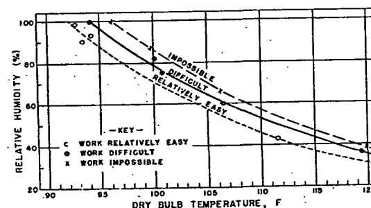
FIG. 3. HEAT ENDURANCE OF ACCLIMATIZED SUBJECTS WORKING AT A SPECIFIC RATE 14
