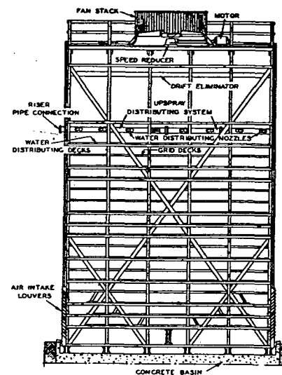
FIG. 8. COUNTERFLOW INDUCED DRAFT COOLING TOWER
