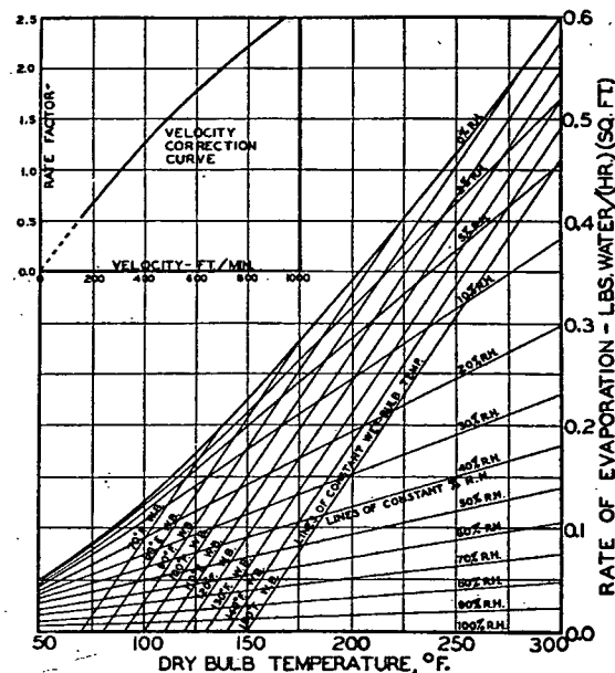
FIG. 8. RATE OF EVAPORATION CHART 3
