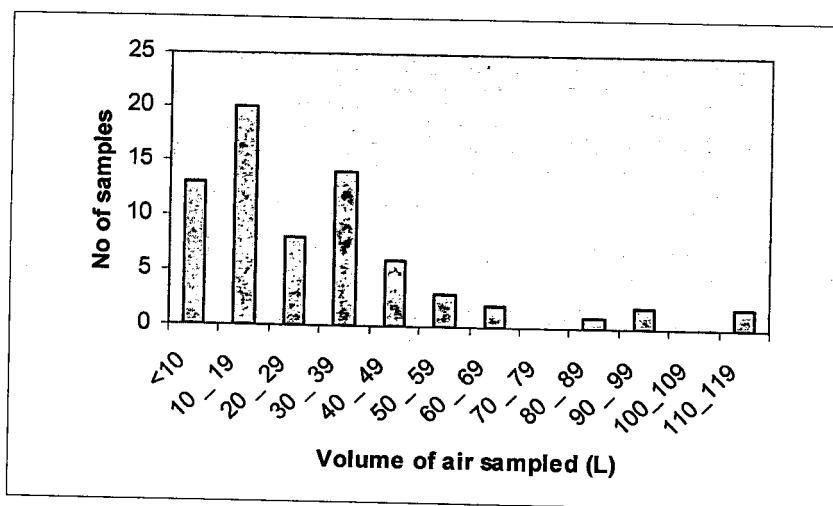
Figure 7: Distribution of sampled air volumes for personal samples counted by PCM.
