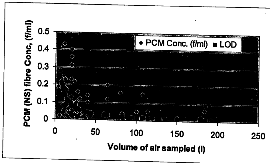
Figure 4: PCM fibre concentrations of treated samples from the HSE/IC study superimposed against the calculated limit of detection (LOD) v volume of air sampled,
