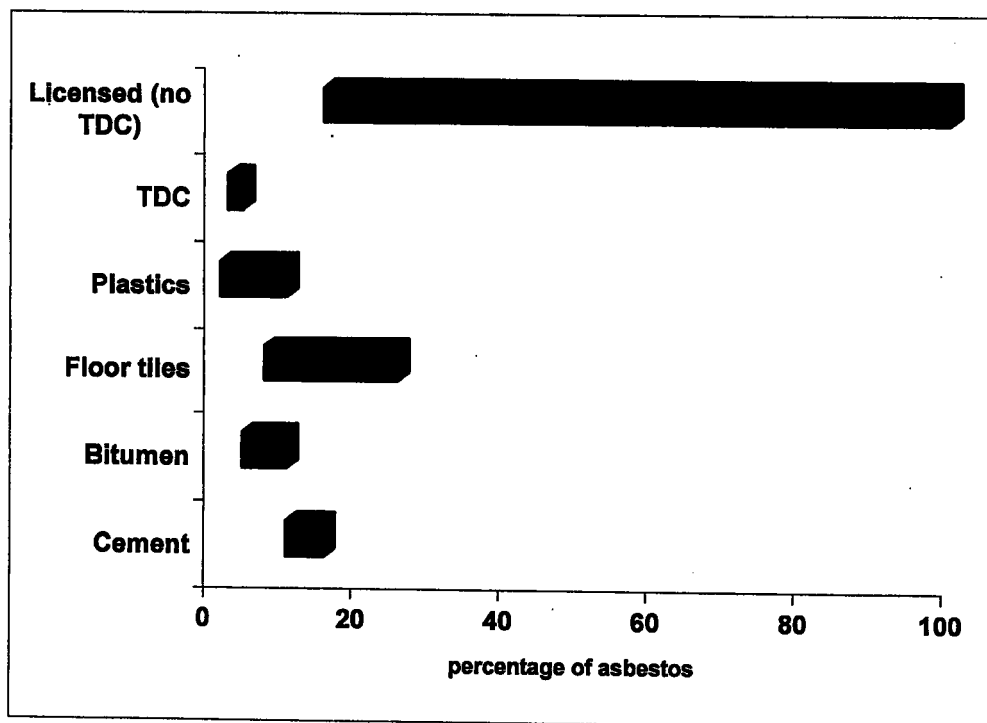
Figure 2: Typical weight percentages of asbestos in licensed and non-licensed asbestos products.
