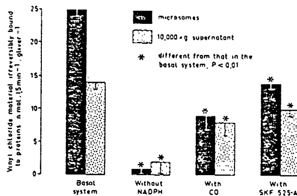
FIG. 4. Irreversible binding of a vinyl chloride material to proteins in vitro . In the basal system, [ 14 C]vinyl chloride (5 mM) was incubated under air with microsomes or 10,000g supernatant from 125 mg of liver from non-pretreated rats and with a NADPH-generating system; in some flasks, the NADPH-generating system was omitted; other flasks were incubated under a 90% CO-10% O 2 atmosphere; in other flasks, SKF 525-A (5 mM) was added to the incubation mixture. After 15 min of incubation, the amount of vinyl chloride material irreversibly bound to microsomal or 10,000g supernatant proteins was measured; columns and bars represent means and SD for three experiments.
