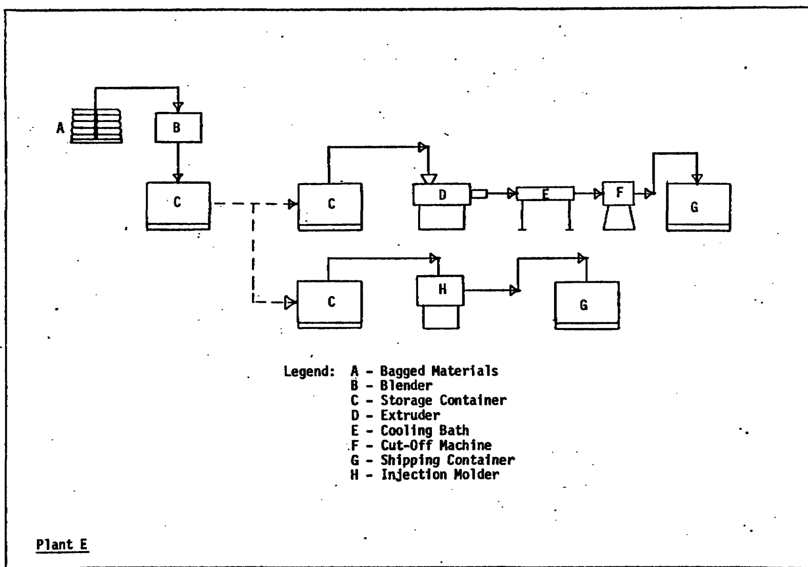
Figure 8. Flow Schematic, Plant E
