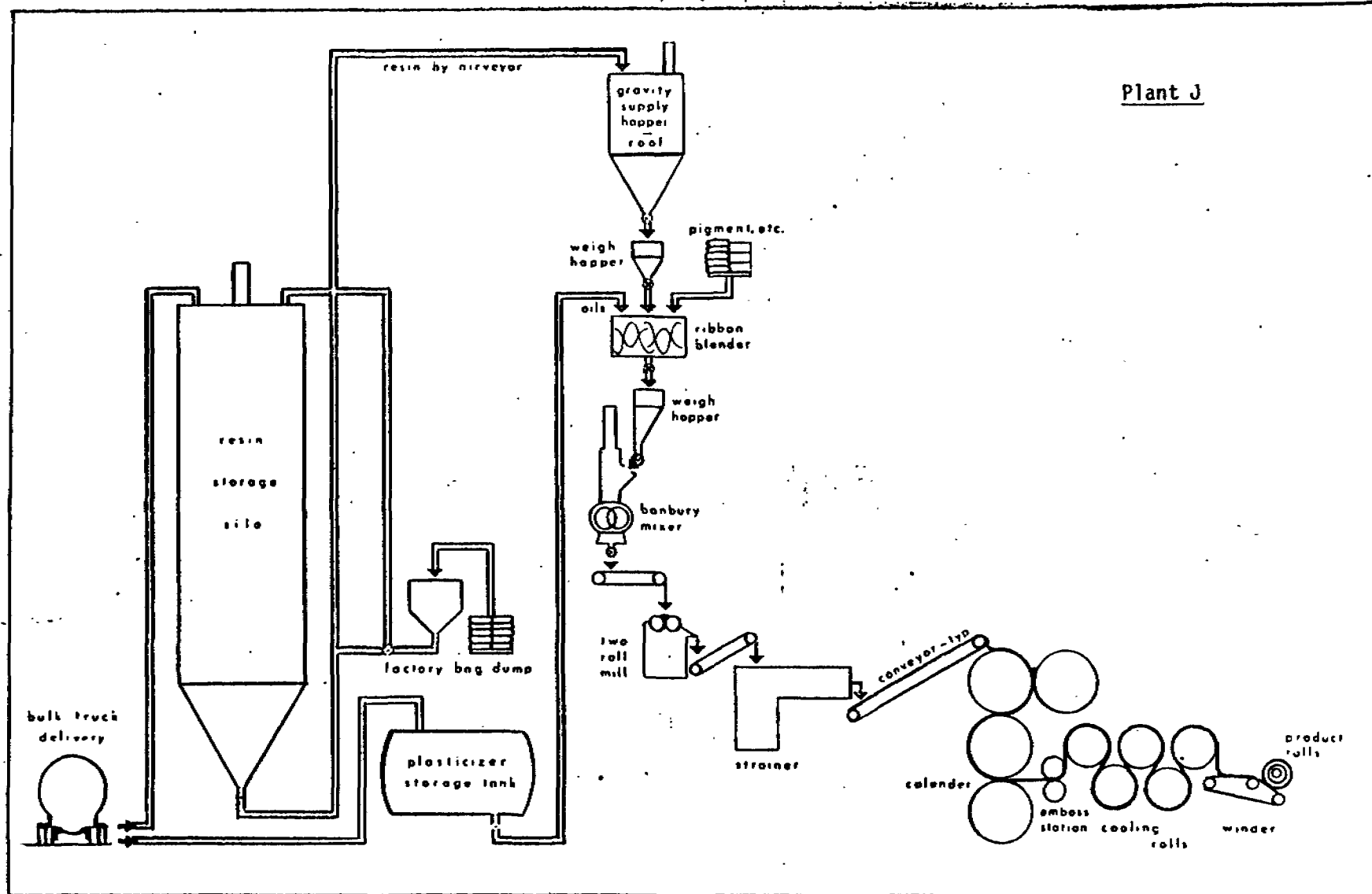
Figure 14. Flow Schematic, Calendered Film Production, Plant J
