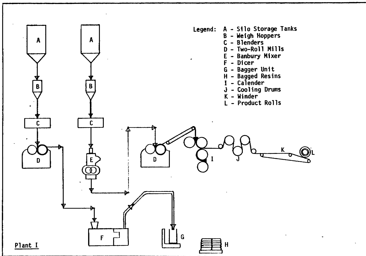
Figure 12. Flow Schematic, Plant I
