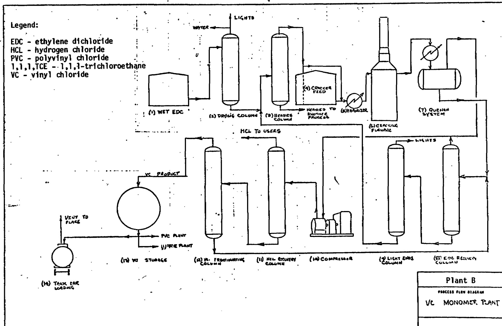
Figure 5. Flow Schematic, Plant B
