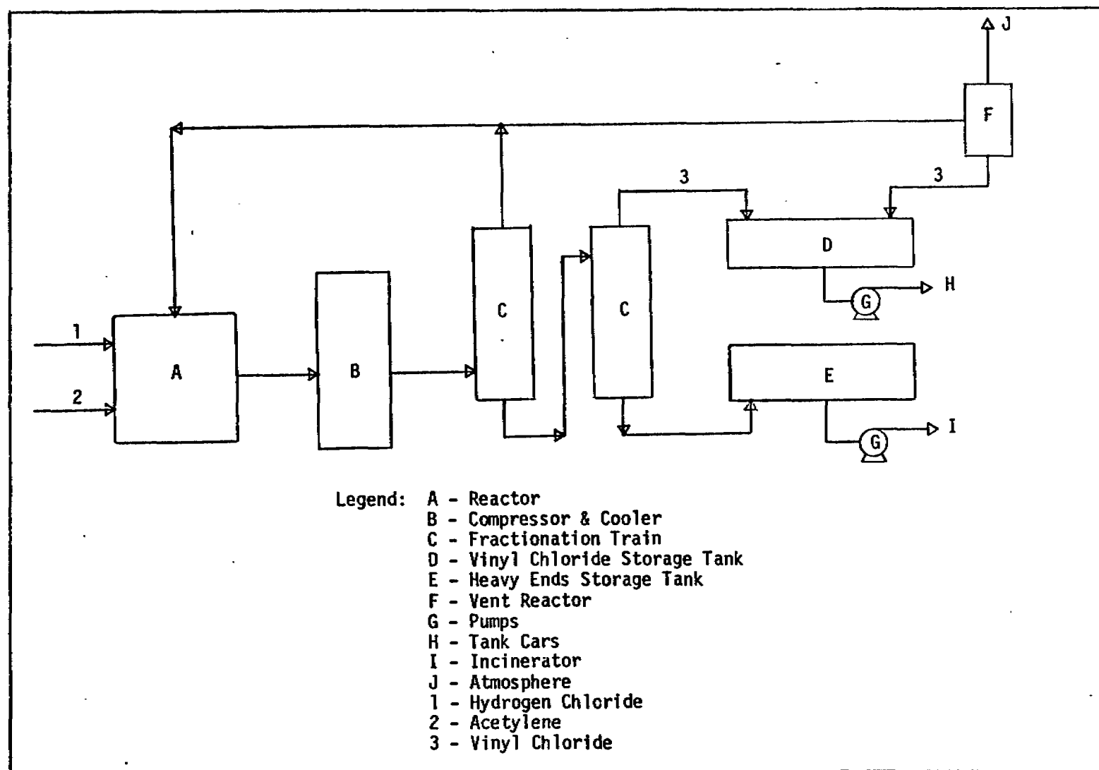
Figure 4. Flow Schematic, Plant A
