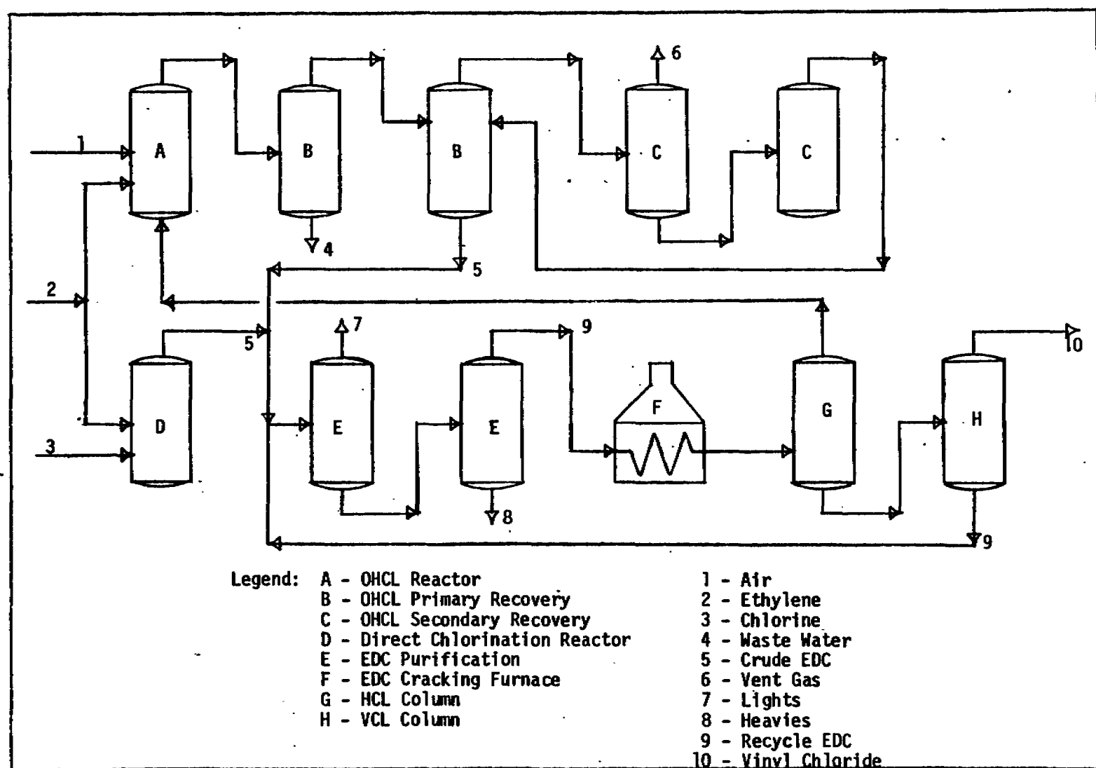
Figure 3. Oxyhydrochlorination Process
