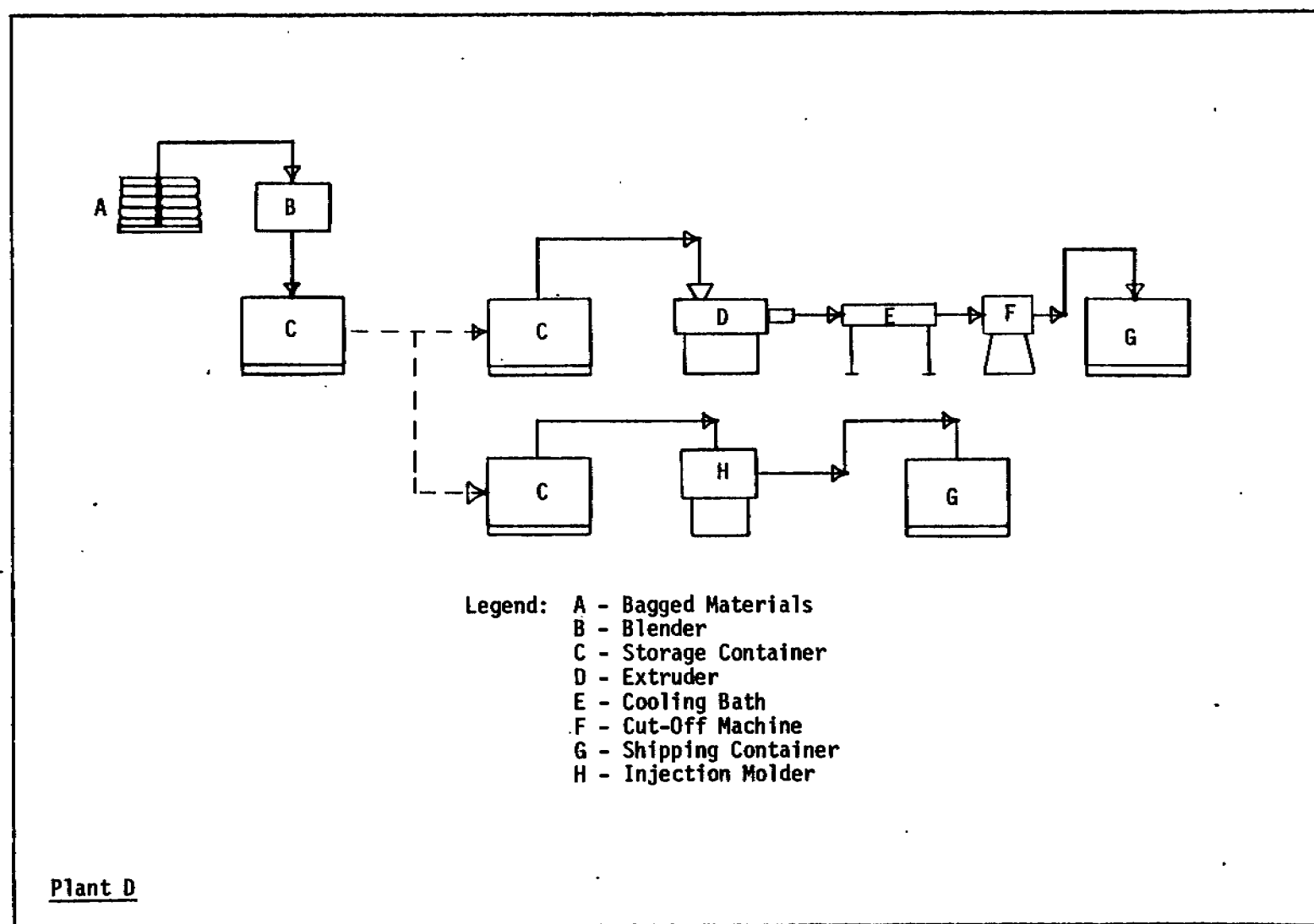
Figure 7. Flow Schematic, Plant D
