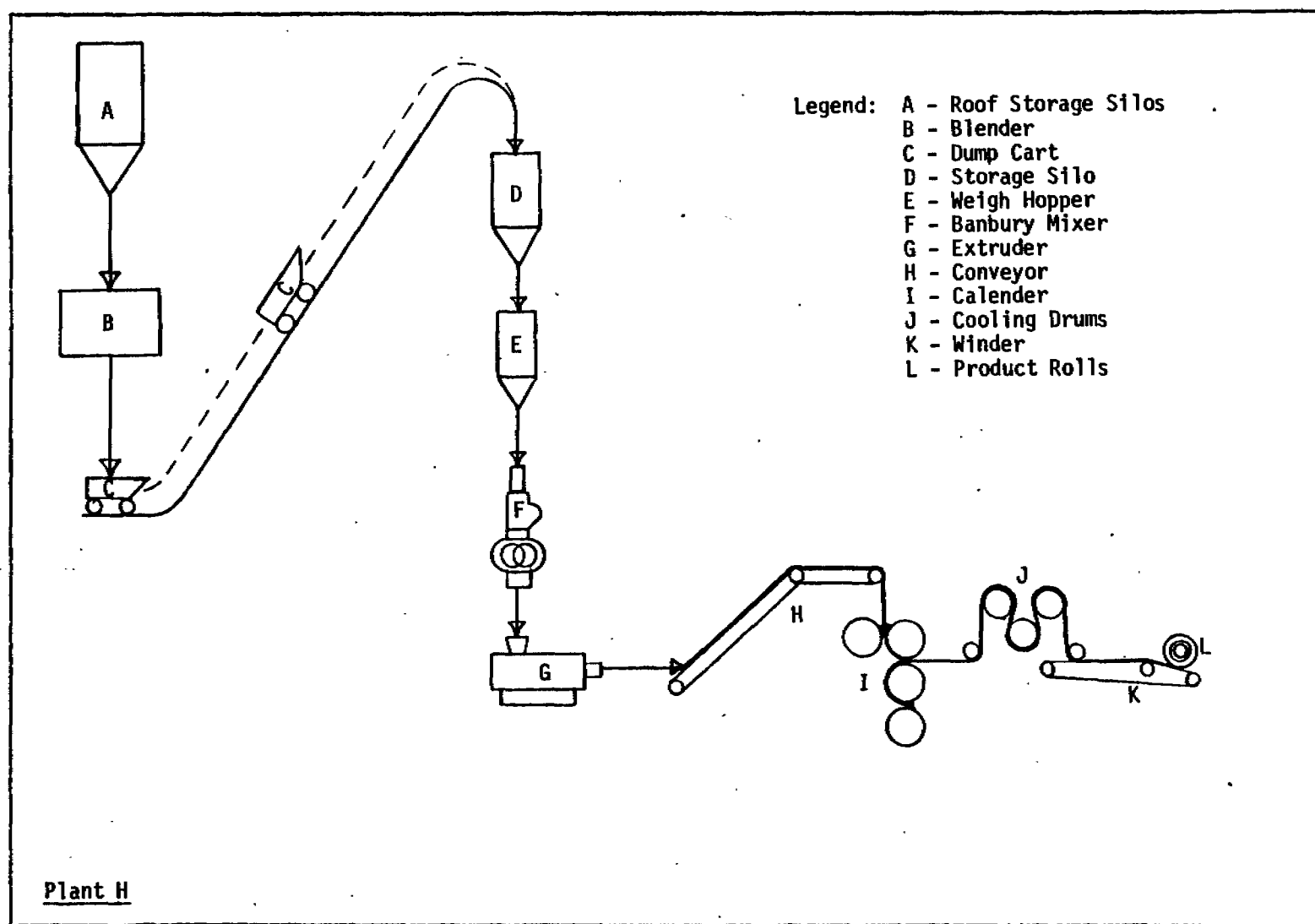
Figure 11. Flow Schematic, Plant H
