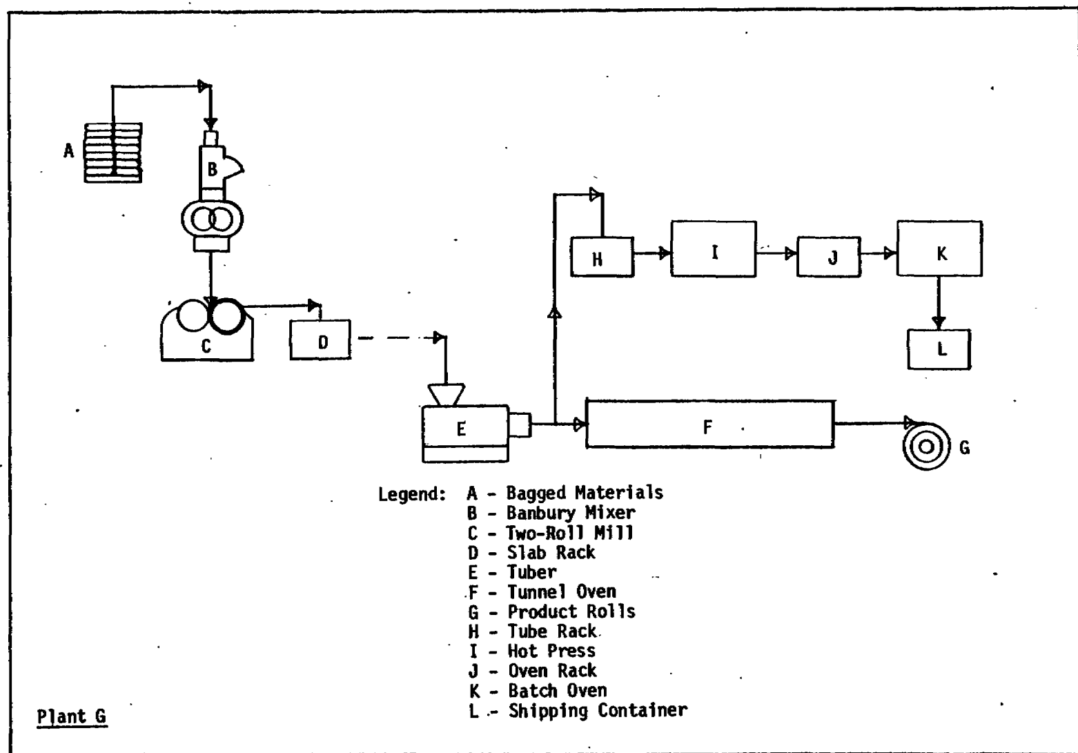
Figure 10. Flow Schematic, Plant G
