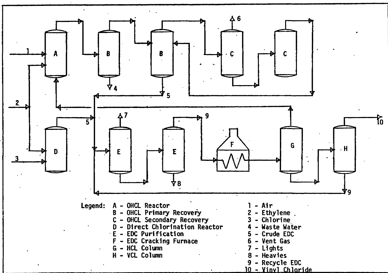
Figure 6. Flow Schematic, Plant C
