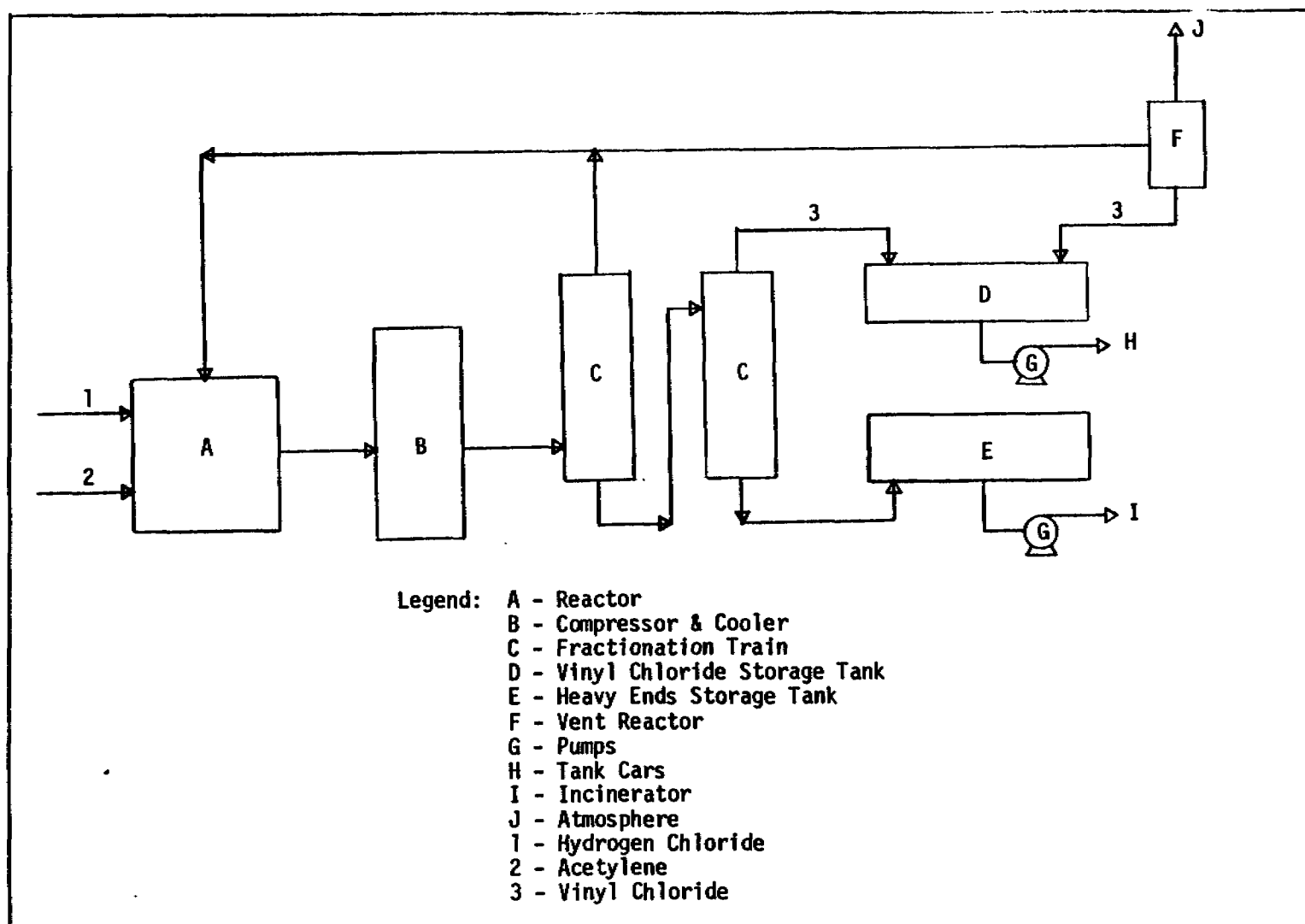
Figure 1. Acetylene-Hydrogen Chloride Process
