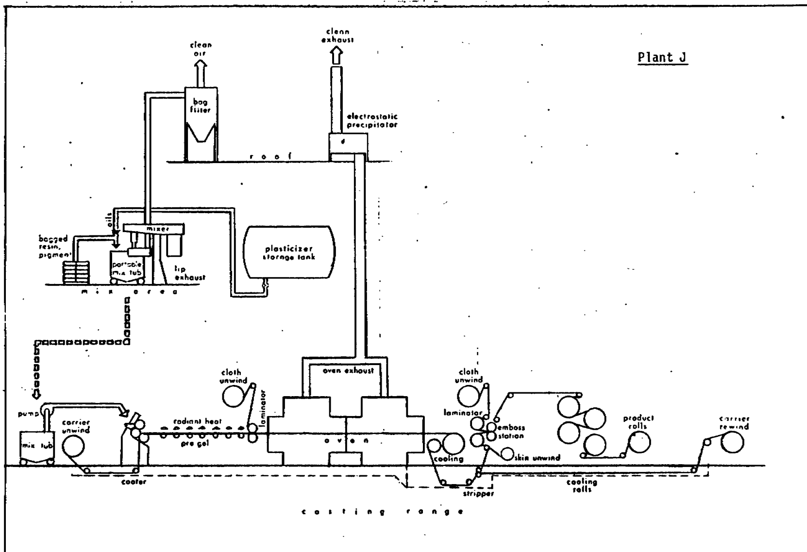
Figure 13. Flow Schematic, Cast Film Production, Plant J
