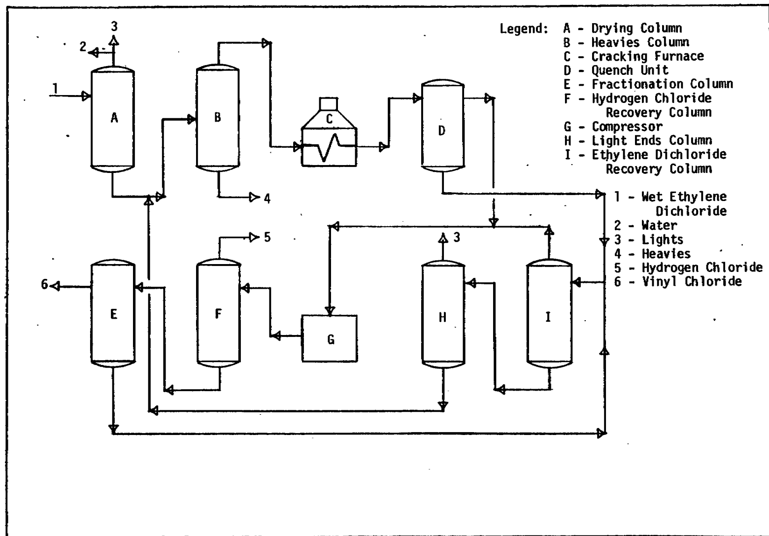
Figure 2. Ethylene Dichloride Pyrolysis Process
