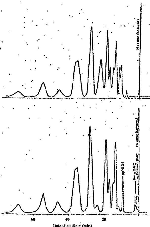
Fig. 1. Gas-liquid chromatograms of (a) extract of kestrel liver and (b) a commercial polychlorobiphenyl resin.
