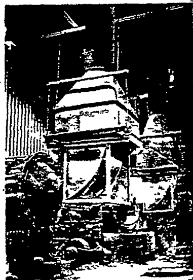
Figure 5 To achieve the proper exhaust air velocity, the hoods for these barrel furnaces can be positioned as close to the furnace spouts as practical. Such positioning is made possible by mounting the hoods on a trolley suspended from an overhead track. (Courtesy American Brake Shoe Co.)
