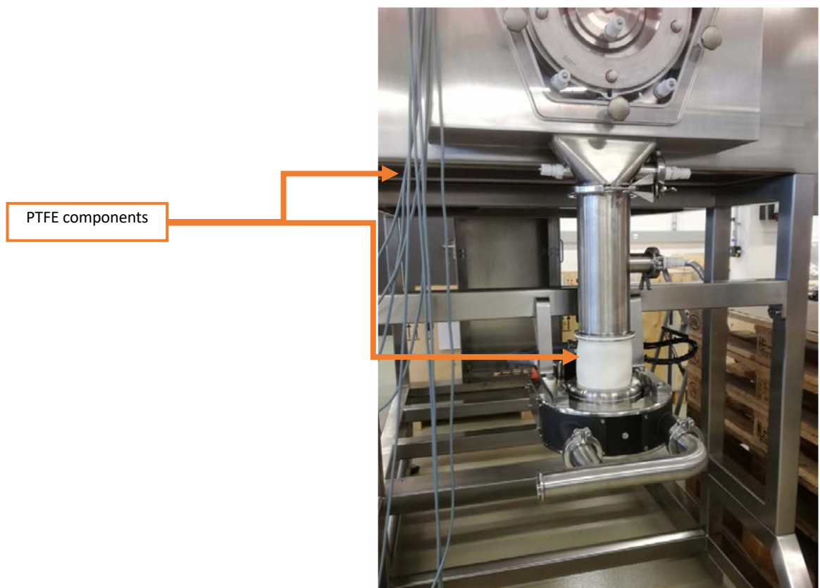
SBV valve powder inlet
