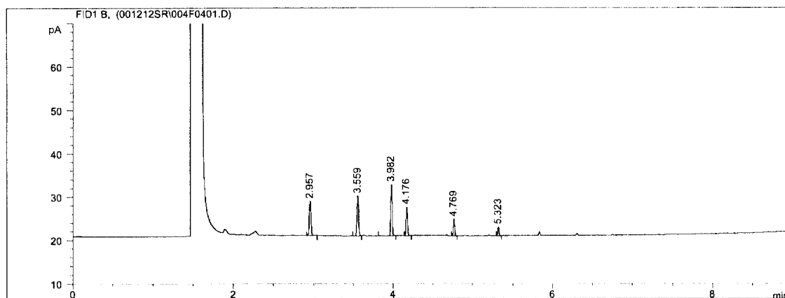
Figure 2c: Representative GC chromatogram of 0.0756 mg/mL H-24516 analytical reference solution.
